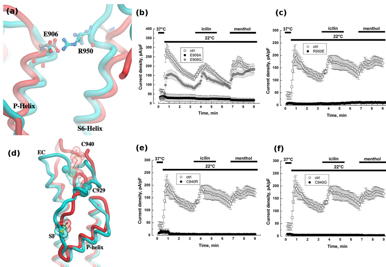
FIGURE 5 Residues involved in conformation of P-helix and of SF-to-S6 EC loop. The closed conformation is colored red and the open state in cyan. The interactions between (a) E 906 and R 950 are rendered as sticks and (d) disulfide bond formed by C 929 -C 940 are illustrated as transparent balls. Whole-cell recordings at +100 mV of TRPM8 currents induced with either cold (22°C), or icilin (10 μM), or menthol (500 μM) for HEK cells transfected with (b) E 906 A or E 906 Q TRPM8 mutant (c) R 950 E TRPM8 mutant (e) C 940 R TRPM8 mutant and (f) C 940 G TRPM8 mutant. Cells transfected with WT TRPM8 were used as control ( ctrl ). To see this figure in color, go online.
