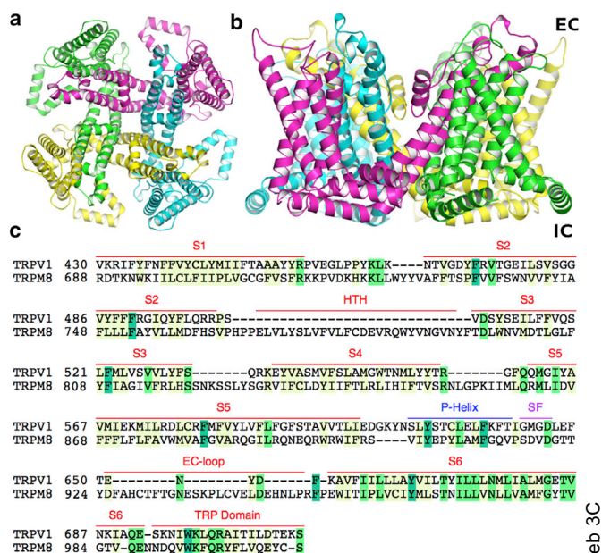
FIGURE 1 (a) Homology model of the human TRPM8 TM region, as viewed from the EC side. Each monomer is colored distinctly. (b) Side view of the human TRPM8 TM region. The IC and EC sides have been labeled. (c) Sequence alignment between the TM regions of human TRPV1 and TRPM8. The regions are labeled above the sequence including the predicted Helix-turn-helix segment (between S2 and S3 helices) and the EC-loop between SF and S6 helix. The colors are based on sequence conservation, where dark green represents total conservation and yellow is partial conservation. The EC and IC sides have been labeled accordingly. To see this figure in color, go online.
