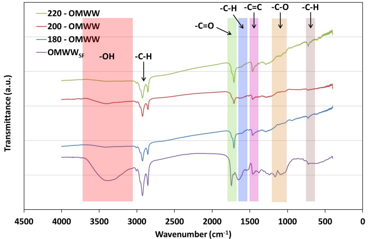
3 4 Figure 6: FTIR specters for the raw OMWW solid fraction (OMWW SF ) and the derived 5 hydrochars produced from raw OMWW at 180°C, 200°C and 220°C
