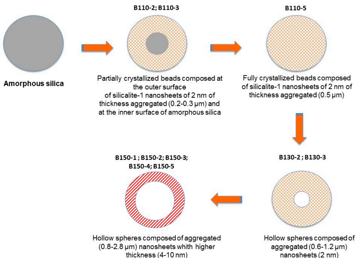
Figure 7. Schematic representation of the pseudomorphic transformation of silica amorphous beads into silicalite-1 beads or hollow spheres composed of silicalite-1 nanosheets samples (B-T( ^{\circ}\text{C} )-t(days)) as a function of the hydrothermal temperature (T in ^{\circ}\text{C} ) and duration (t in days).
