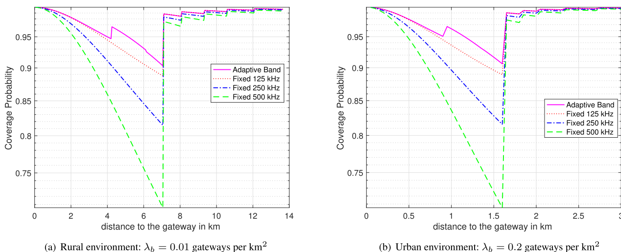
FIGURE 4. Variation of coverage probability with distance.
