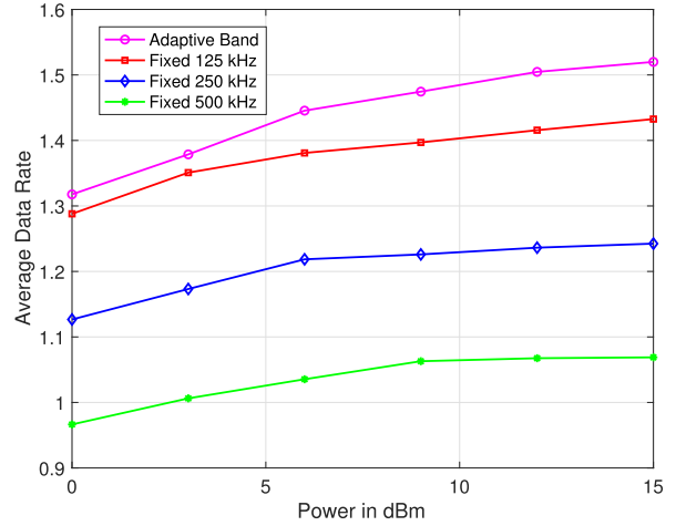
FIGURE 8. Average data rate in kb/s versus the device power - Rural environment \lambda_b = 0.01 gateways per \text{km}^2 .
