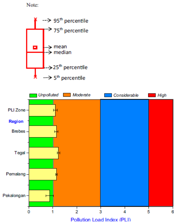
Fig. 3 Pollution load index (PLI) of the metals in the sediments of the studied area
