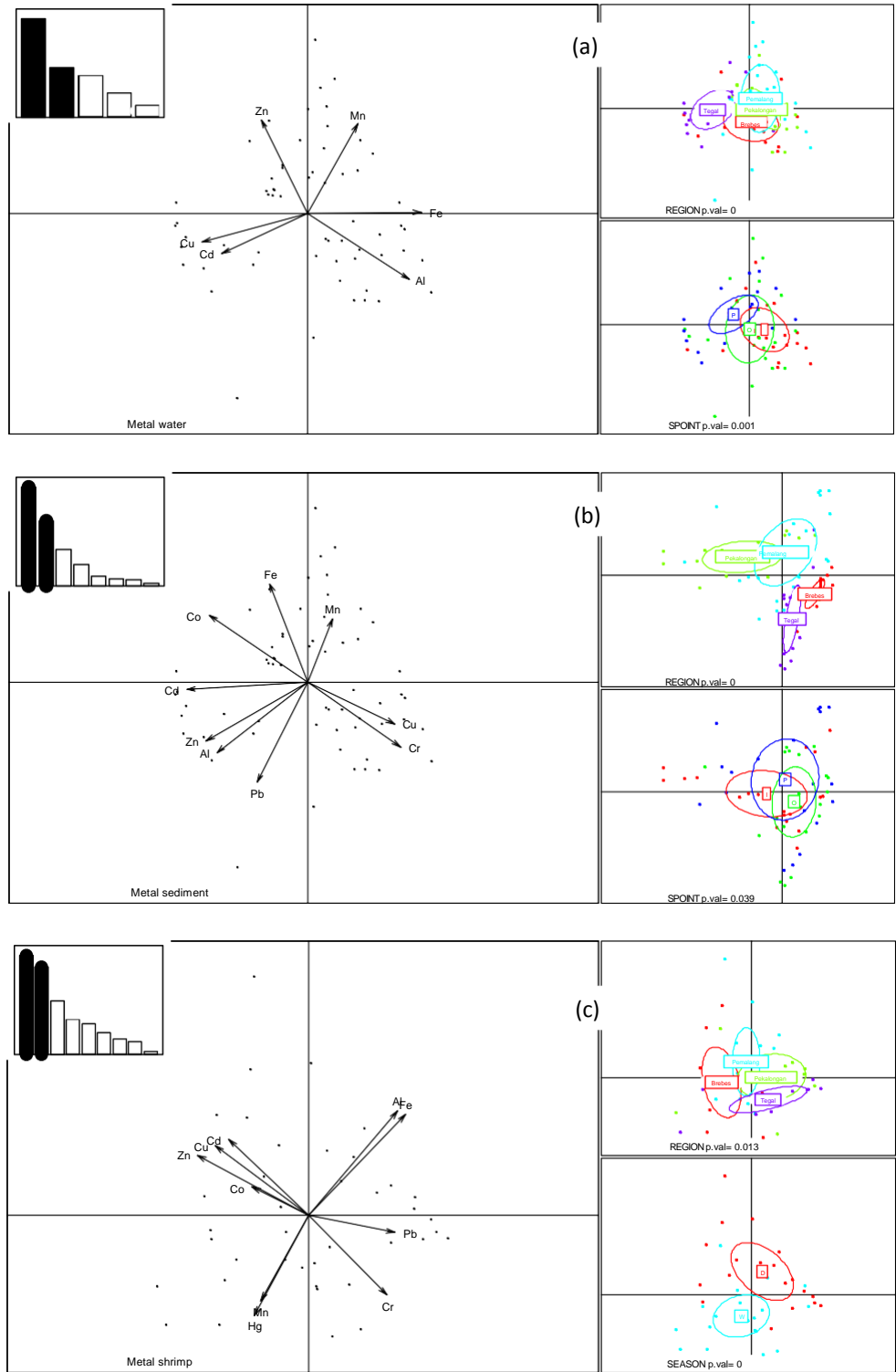
Fig. 4 Principal component analysis of the metals in a water, b sediment, and c shrimp
