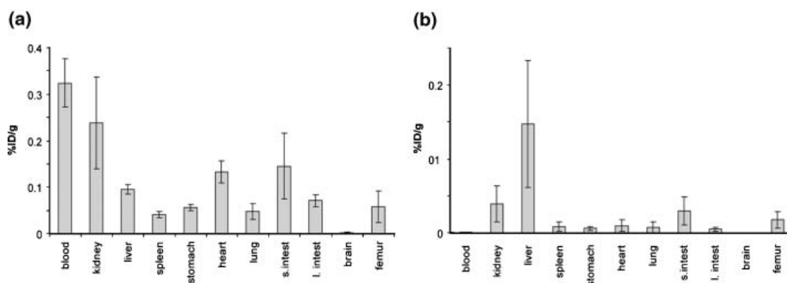
Figure 7. Biodistribution, stated as percentage of injected dose per gram of organ (%ID/g \pm SD), of ^{153}\text{Sm}_3\text{L} in Wistar rats: (a) 15 min and (b) 1 h after intravenous injection. Results are the mean values of four animals.
