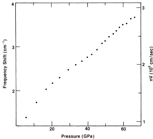
FIG. 1. Measured Brillouin frequency shift from longitudinal sound waves in \text{H}_2\text{O} as a function of pressure.
