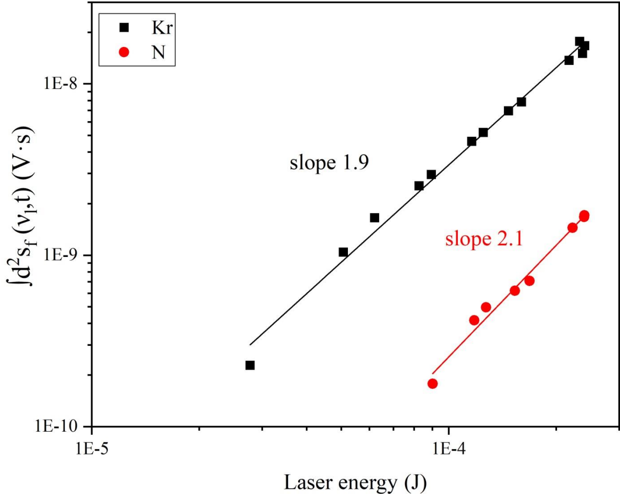
Figure 7: Measured variations of the time-integrated TALIF signal intensities as a function of the laser energy for nitrogen and krypton. For these measurements, the laser frequency was set at the peak of absorption ( \nu_1 = \nu_A/2 ).
