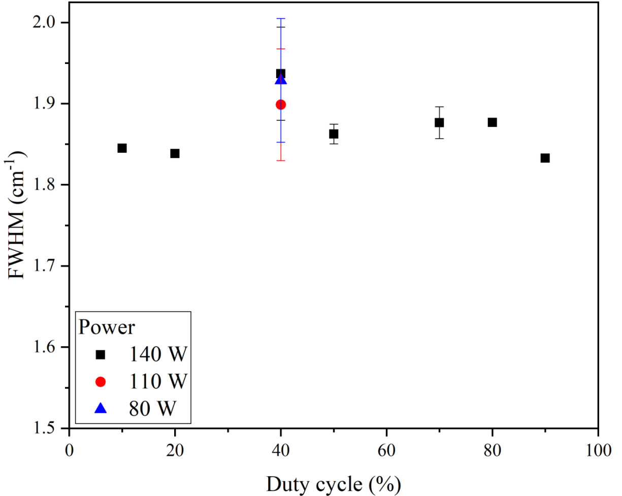
Figure 2: Experimental spectral width of the excitation spectrum \Delta\nu_{G,N}^{eff} in \text{cm}^{-1} , measured at the fundamental wavelength of the dye laser ( 16125.135 \text{ cm}^{-1} ), and deduced from the laser excitation spectra for several duty cycles and three MW powers.
