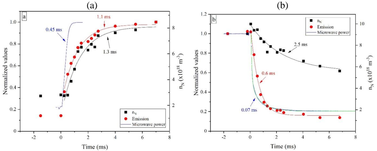
Figure 10: Temporal evolution of the N(^4S) -atom density, the N_2(B) emission and the MW power for (a) high power phase and (b) low power phase at pressure of 20 pa and 50% duty cycle. The time origin, t = 0 , is chosen at the start of the power increase (a) or decrease (b) when transitioning between the high and low power phases. .
