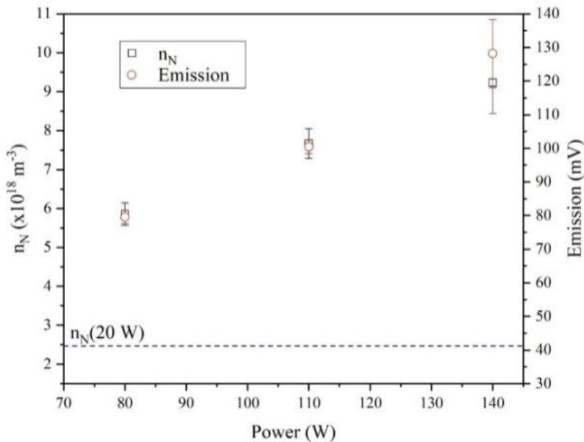
Figure 9: Influence of the peak MW power on the N-atom densities deduced from TALIF measurements (black open squares) and on the 728-750 nm FPS emission (red open circles) as a function of the coupled MW power.
