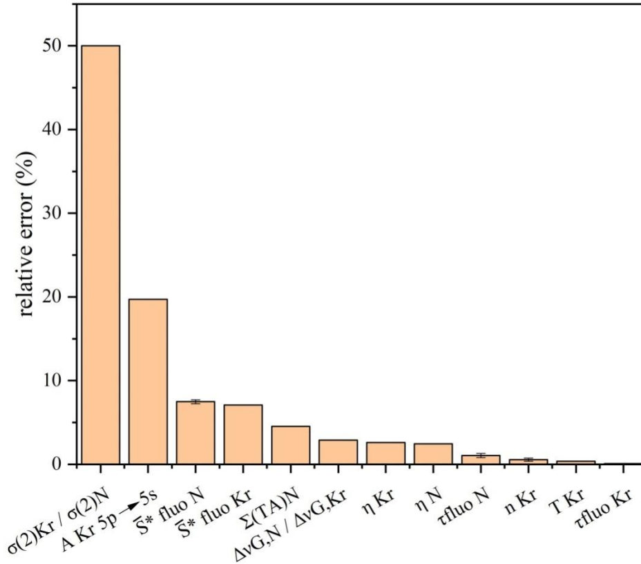
Figure 6: relative errors for the different terms of the equation (14)
