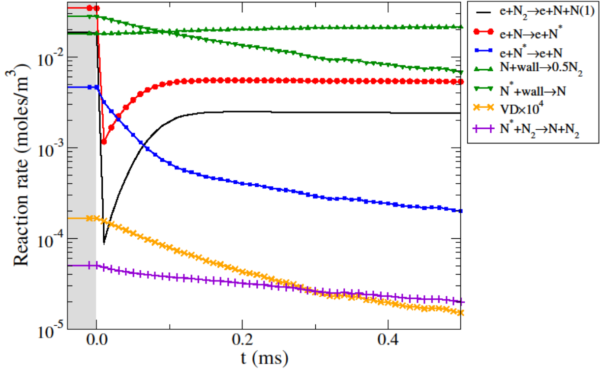
Figure 14 : Time-variation of the main electron impact processes involved in the kinetics of N(^4S) -atom at the transition between the high- and low-power phases. The rate of surface recombination processes are also shown for comparison.
