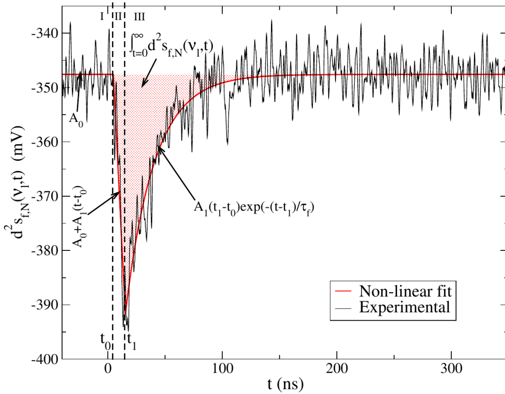
Figure 3: A sample raw PMT signal (black line) and the corresponding fit, indicating the three regions of the signal and the corresponding temporal integral of the signal \int_{t=0}^{\infty} d^2 s_{f,N}(v_l, t) .
