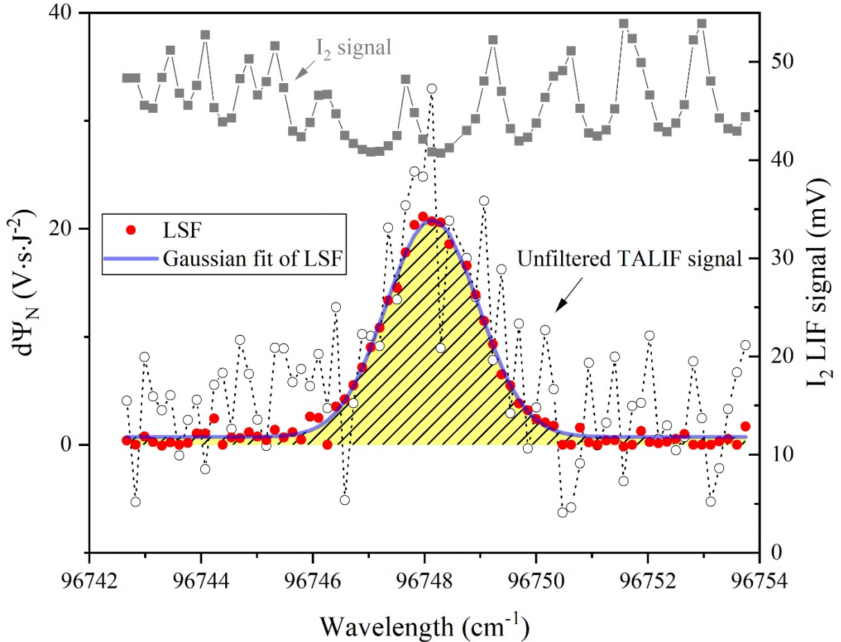
Figure 4: N TALIF absorption spectra from raw data (black open circles), data processed using the program (red solid circles) and these data fitted with a Gaussian function (blue line). The pressure is equal to 20 Pa and the maximum MW power is equal to 140 W. The I_2 LIF
