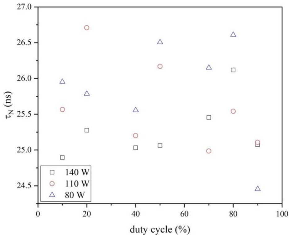
Figure 5: Decay time of N-atom fluorescence as a function of the duty cycle for different average input power values. The estimated mean value of N(4S) life-time was assessed to be 26 \pm 1.4 ns.
