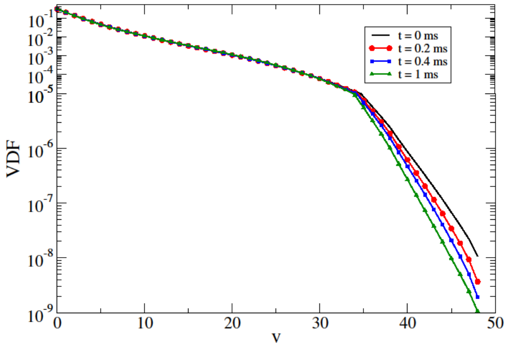
Figure 13 : Time-variation of the vibrational distribution functions during the transition to the low power phase. The simulation was performed for a pressure of 20 Pa, a power density of 1 \text{ W.cm}^{-3} , a pulse period of 100 ms and a duty cycle of 0.5. The emphasis is put on the high/low power transition.
