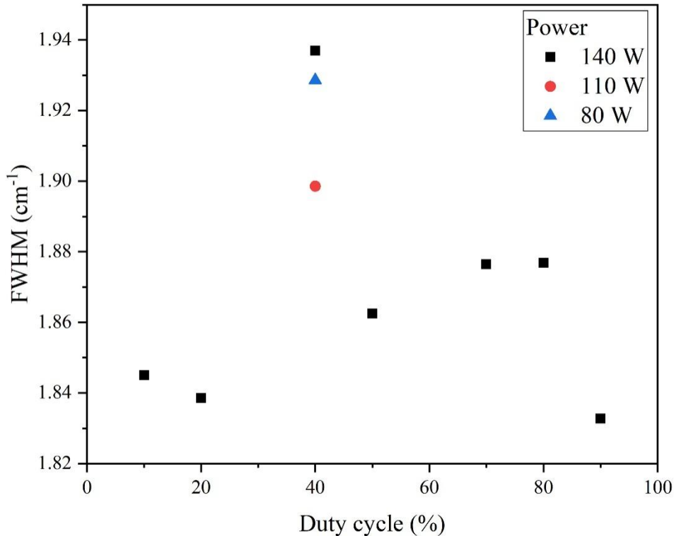
Figure 2: experimental spectral width in \text{cm}^{-1} , measured at the fundamental wavelength of the dye laser ( 16125.135 \text{ cm}^{-1} ), and deduced from the laser excitation spectra for several duty cycles and three MW powers.
