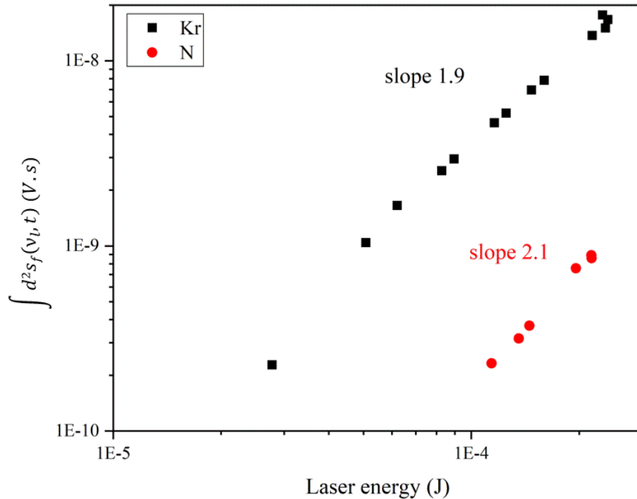
Figure 7: Measured variations of the time-integrated maximum intensity of the TALIF signal as a function of the laser energy for nitrogen and krypton.
