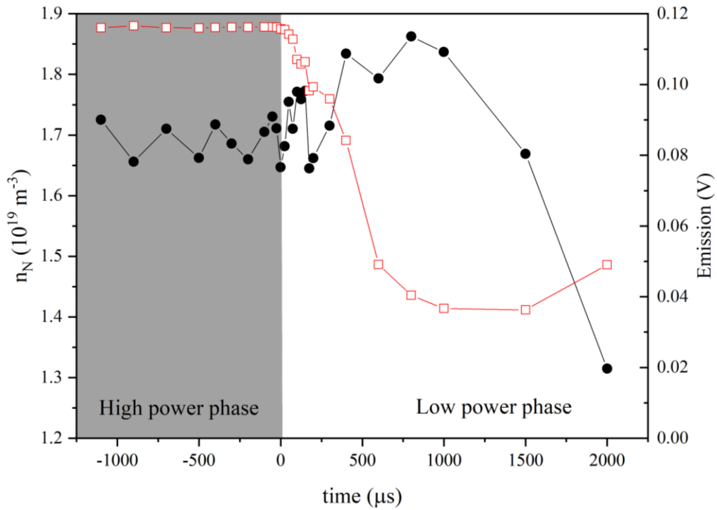
Fig 11: Time-resolved measurement of N -atom and N_2(B^3\Pi_g) emission around the transition between the high and low power phases and during the early stage of the low power phase..
