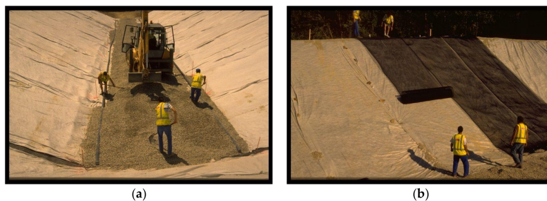
Figure 4. (a) Bottom and; (b) lateral watertight during the placement.
