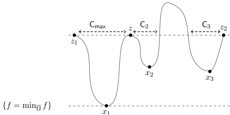
Figure 6: A one dimensional case when (A0) , (A1) , (A2) , and (A3) are satisfied with C = \{C_{\max}, C_2, C_3\} . The assumption (A4) is not satisfied because \partial C_{\max} \cap \partial C_2 = \{z\} \neq \emptyset .
