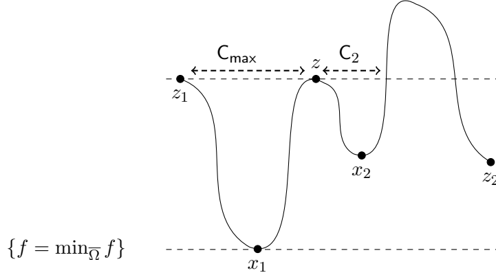
Figure 5: A one dimensional case when (A0) , (A1) , and (A2) are satisfied with \mathcal{C} = \{C_{\max}, C_2\} . The assumption (A3) is not satisfied because \partial C_{\max} \cap \partial \Omega = \{z_1\} and f(z_1) > f(z_2) = \min_{\partial \Omega} f .
