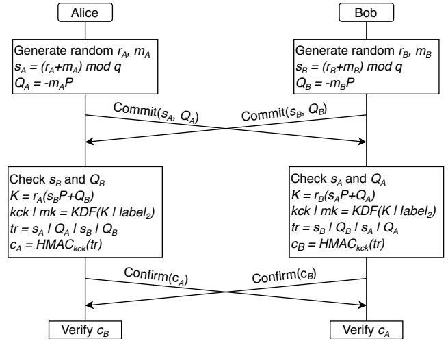
Figure 1: Dragonfly handshake workflow. P is the group element derived from the password, and \text{label}_2 is a string that may vary along with the protocol in which the handshake is performed.
