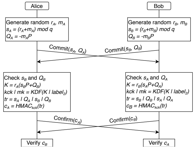
Figure 1: Dragonfly handshake workflow. P is the group element derived from the password, and \text{label}_2 is a string that may vary along with the protocol in which the handshake is performed.
