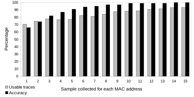
Figure 2: Reliability of our experiment given a different number of samples to interpret for each MAC address. Accuracy represents the closeness of our prediction to the real value. Usable traces represent the percentage of traces we were able to automatically exploit, without high risk of miss-prediction.
