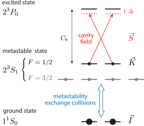
FIG. 2. Relevant level scheme of ^3\text{He} for z quantization axis, which corresponds to the cavity axis. The cavity mode (red) addresses the C_8 transition between the F = 1/2 metastable manifold and the F = 1/2 excited state 2^3P_0 , with detuning \Delta . The six metastable levels 2^3S_1 are coupled to the purely nuclear 1^1S_0 ground state by metastability exchange collisions.
