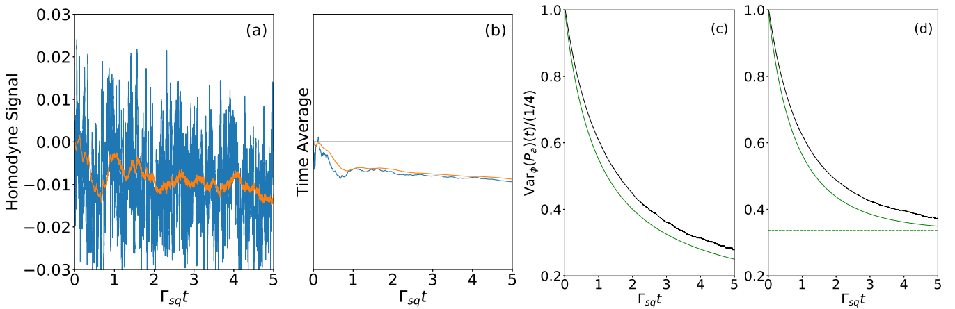
FIG. 3. (a) Time evolution of the homodyne signal \langle c + c^\dagger \rangle_\phi (blue) and of the nuclear spin quadrature 2\sqrt{\frac{\Gamma_{\text{sq}}}{\kappa}} \langle P_a \rangle_\phi (orange) in a single realization of the experiment where a continuous homodyne measurement of the y -polarized field leaking out of the cavity is performed. (b) Time average of the same quantities. The curves are obtained from the continuous stochastic equation derived from the three-mode QME (6), for a single realization of the stochastic noise describing homodyne detection (the equivalent of d\zeta_s of the one-mode model) and averaged over 5 realization of the stochastic noise describing metastability exchange. Parameters: \Omega/\kappa = 1/10 , \gamma_m/\kappa = 1/10 , \gamma_f/\kappa = 1/100 , \Gamma_{\text{sq}}/\kappa = 1/1000 . (c) Conditional variance of the nuclear spin quadrature P_a as a function of time. Black: three-mode model with same parameters as (a), Green: analytical prediction (13) of the one-mode model. (d) Effect of decoherence. Black: three-mode model with an additional relaxation rate \gamma_0/\kappa = 1/1000 in the metastable state, where we now average over 8 realizations of the stochastic noises related to metastability exchange and wall relaxation in the metastable state. Green: one-mode model with the corresponding effective relaxation in the ground state \gamma'_0 = \Gamma_{\text{sq}}/10 . Dashed horizontal line: analytical prediction (16).
