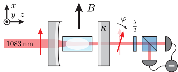
FIG. 1. Illustration of the proposed setup. A Helium-3 vapor cell is placed inside an asymmetric optical cavity, ensuring that photons leave the cavity at rate \kappa predominantly through the out-coupling mirror. A (switchable) discharge maintains a small fraction of the atoms in a metastable state. The atomic metastable and nuclear spins are oriented in the x direction beforehand by optical pumping. The light polarization, initially along x , is rotated by an angle \varphi due to the Faraday effect, performing a quantum nondemolition measurement of the nuclear spin fluctuations along the light propagation direction. This polarization rotation is continuously monitored via homodyne measurement.
