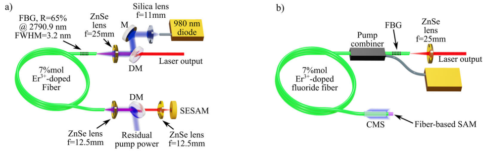
Fig. 1. a) Experimental setup of the mode-locked Er 3+ -doped fiber laser based on a SESAM and an FBG. b) Proposed experimental setup for the mode-locked Er 3+ -doped fiber laser based on a SA fiber and an FBG. (CMS: cladding mode stripper, DM: dichroic mirror, M: gold mirror)
