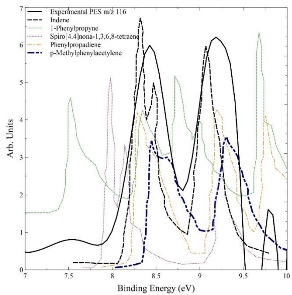
Figure 16. Photoelectron spectra for m/z 116 (experimental) and selected isomers (indene [85], 1-phenylpropyne [86], spiro[4.4]nona-1,3,6,8-tetraene [86], phenylpropadiene [87], p-methylphenylacetylene [88]).
