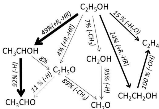
Figure 9. Integrated rates of production, 2.7% C_2H_5OH in argon, T_0 = 1232 K, P_0 = 7.4 bar. The percentages refer to the consumption of the reactant species, the arrow thickness is proportional to the corresponding flux. CRECK model [70].
