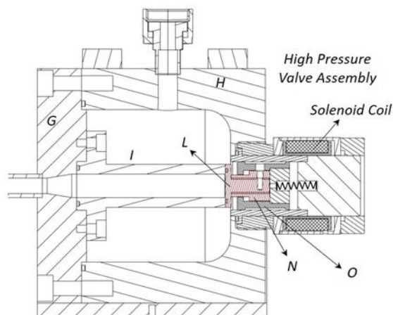
Figure 2: Cross-sectional view of the driver section showing the high-pressure chamber and solenoid actuated valve. G: flange with convergent section; H: main chamber body; I: leading part of the driven section; L: poppet; N: outer body; O: armature body. Parts L, N and O form the armature.
