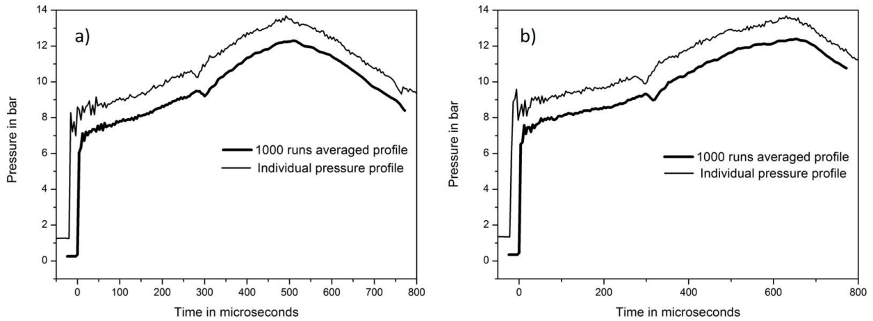
Figure 3. Pressure time-histories for a single experiment and an average pressure over 1000 experiments for the following conditions: a) T_5 = 1509 K, P_5 = 7.3 bar; b) T_5 = 1297 K, P_5 = 7.8 bar. For clarity, the individual pressure profiles are offset relative to the averaged profile (+1 bar, -20 \mu s). Without the offset, the profiles would be largely indistinguishable.
