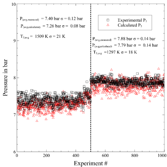
Figure 4. Distribution of measured and calculated reflected shock pressures using extrapolated velocities to the end-wall of the shock tube.
