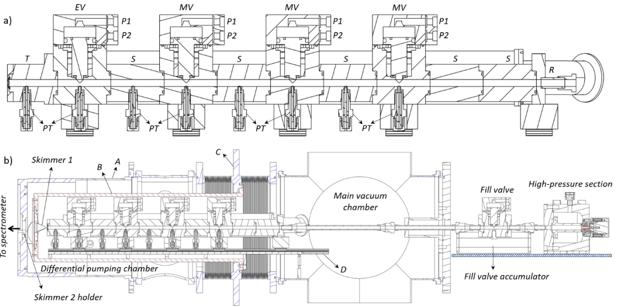
Figure 1: a) Cross-sectional view of the part of the driven section of the ICARE-HRRST that sits inside the SAPHIRS vacuum chamber at SOLEIL. The part that connects R to the vacuum feedthrough is a section of tube and is not shown. EV : end valve; MV : middle valves; T : end section; S : spacers; R : connection element; PT : pressure transducer holders. Compressed air is connected to ports P1 and P2 . b) ICARE-HRRST coupled with DESIRS-SAPHIRS. A : DESIRS-SAPHIRS outer chamber; B : DESIRS-SAPHIRS inner chamber; C : movable support flange for chamber B ; D : slab with linear guides. Cross-sectional view of the ICARE-HRRST with part of the driven section.
