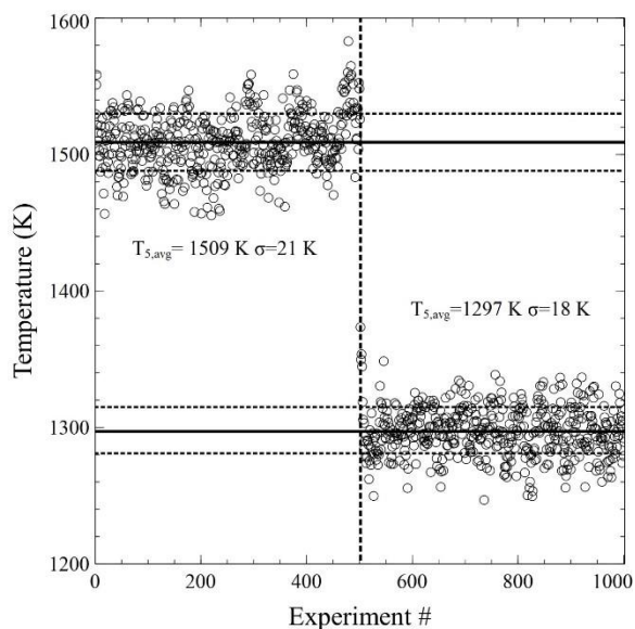
Figure 5: Distribution of calculated reflected shock temperatures using extrapolated velocities to the end-wall.
