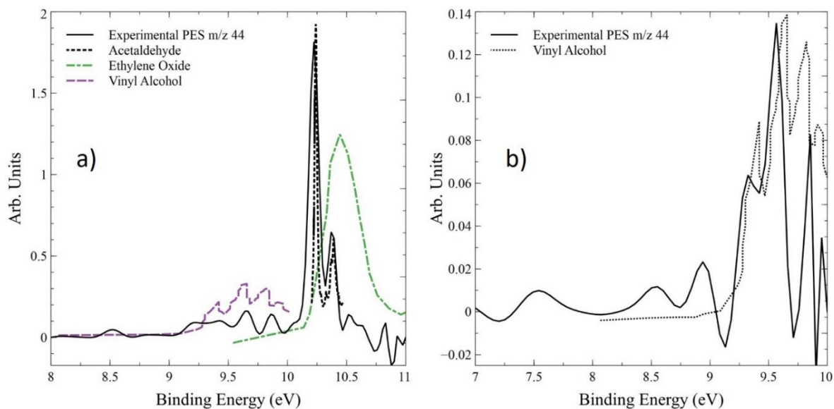
Figure 12. Photoelectron spectra for m/z 44 (experimental), acetaldehyde [35], ethylene oxide [76] and vinyl alcohol [35]. Photon energy equal to a) 11.0 eV, b) 10.0 eV.
