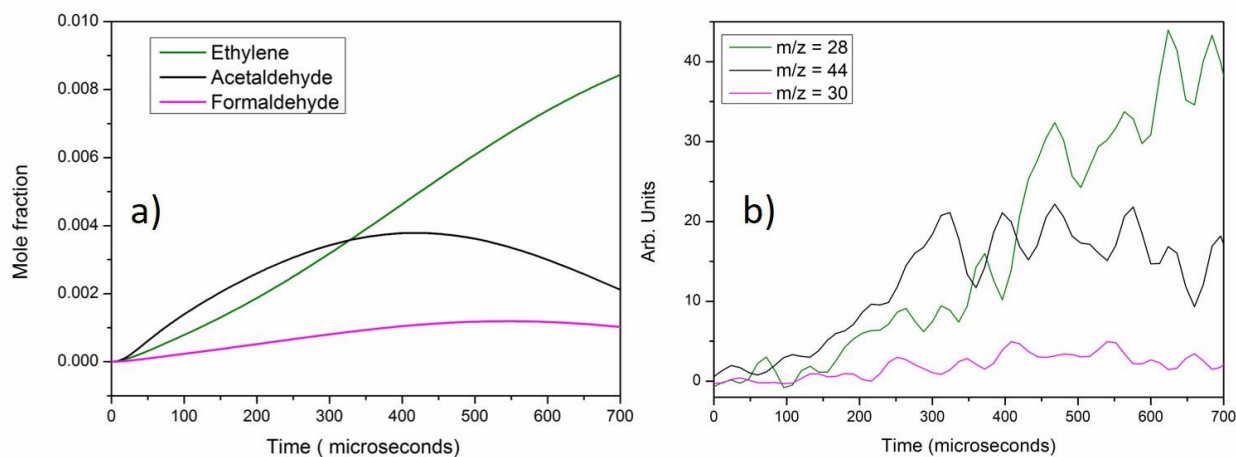
Figure 10. Time histories for ethylene and m/z 28 (green), acetaldehyde and m/z 44 (black) and formaldehyde and m/z 30 (pink). a) Simulations with CRECK model [70]; b) experimental profiles.
