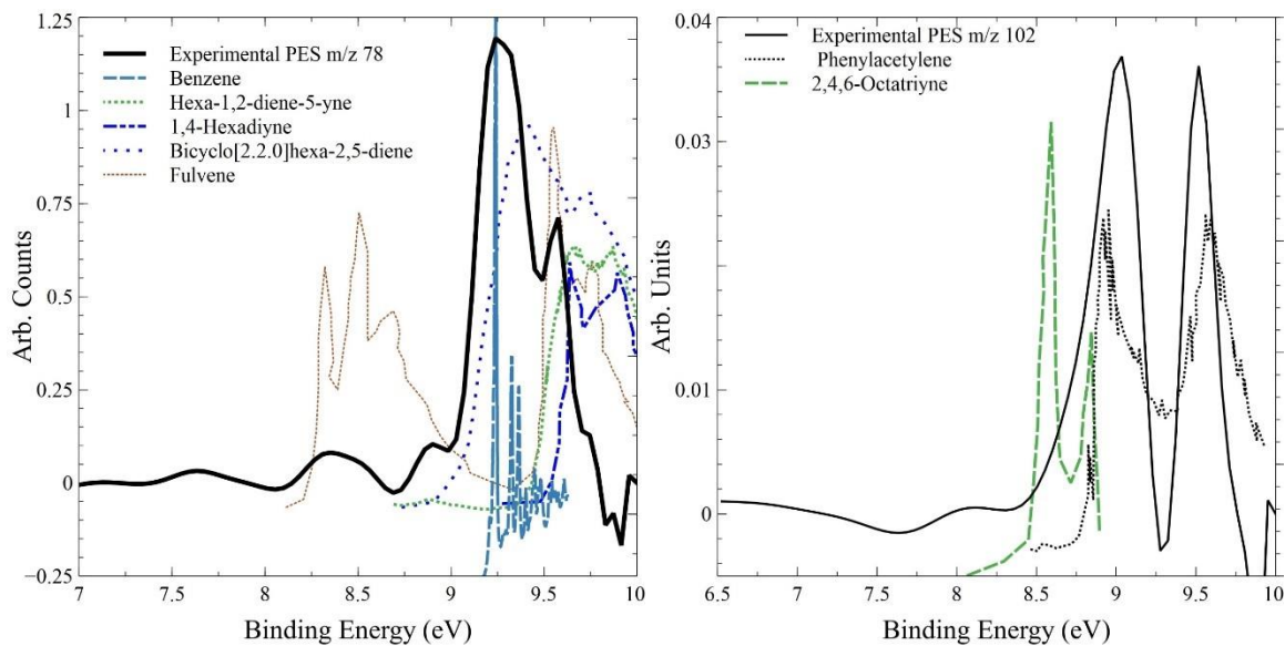
Fig 15. a) Photoelectron spectra for m/z 78 (experimental), benzene [78], fulvene [79], 1,2-hexadiene-5-yne [80], 1,4-hexadiyne [81], and bicyclo[2.2.0]hexa-2,5-diene [82]. b) Photoelectron spectra for m/z 102 (experimental), phenylacetylene [83], and 2,4,6-octatriyne [84].
