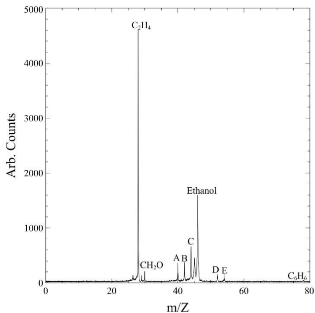
Figure 6: Mass spectrum obtained in Case 1. A: propyne, B: propene/ketene, C: acetaldehyde+ vinyl alcohol, D: vinylacetylene, E: 1,3 butadiene (possible contribution from 1-butyne). Photon energy 11.0 eV.
