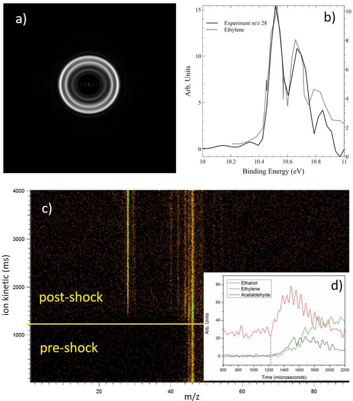
Figure 7: a) photoelectron image corresponding to m/z 28; b) comparison of photoelectron spectra for m/z 28 (experimental) and ethylene [62]; c) ion kinetics for each mass, horizontal line distinguishes the pre-shock and post shock region; d) temporal profiles of ethanol (red), ethylene (green), and acetaldehyde (black), with a vertical line distinguishing pre-shock and post-shock area. The experimental profiles were obtained by taking vertical slices from Fig. 7c.
