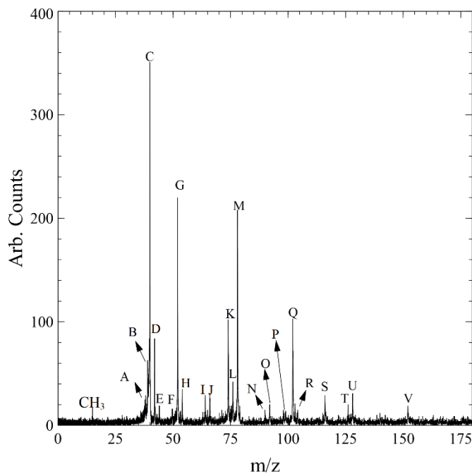
Figure 14: The mass spectrum obtained from the case 3 study. A: m/z 38, B: propargyl radical, C: allene, D: propene/ketene, E: vinyl alcohol, F: m/z 50, G: vinylacetylene, H: 1,3 butadiene/2-butyne, I: 1,3-pentadiyne, J: cyclopentadiene, K: triacetylene, L: m/z 76, M: benzene, N: m/z 90, O: m/z 92, P: m/z 98, Q: phenylacetylene, R: styrene, S: indene/ p -methylphenylacetylene, T: m/z 126, U: m/z 128, V: m/z 152. Photon energy 10.0 eV.
