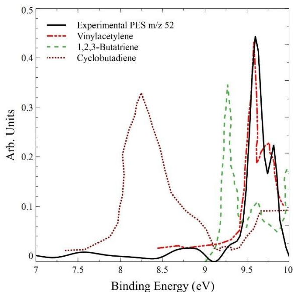
Figure 13. Photoelectron spectra for m/z 52 (experimental), vinylacetylene [63], 1,2,3-butatriene [64], and cyclobutadiene [65]. Photon energy equal to 10.0 eV.
