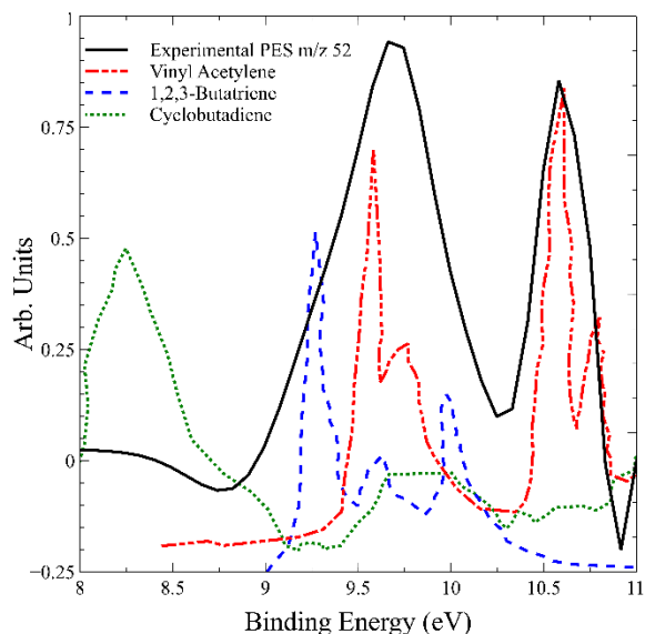
Figure 8. Photoelectron spectra for m/z 52 (experimental), vinylacetylene [63], 1,2,3-butatriene [64], and cyclobutadiene [65]. Photon energy equal to 11.0 eV.
