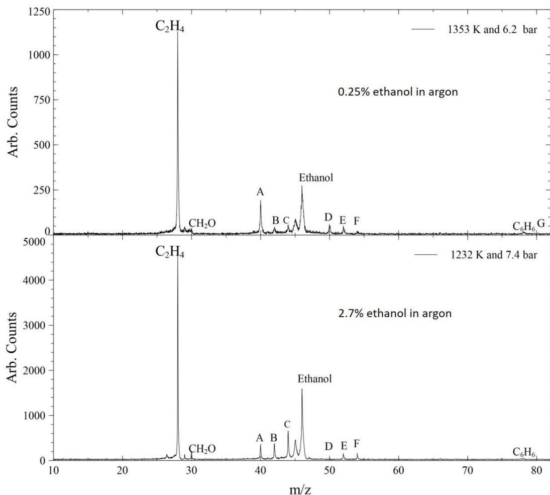
Figure 17. (Top) Mass spectrum obtained with 0.25% ethanol in argon. A: propyne, B: propene/ketene, C: acetaldehyde+ vinyl alcohol, D: diacetylene, E: vinylacetylene, F: 1,3 butadiene (possible contribution from 1-butyne). (Bottom) Mass spectrum obtained with 2.7% ethanol, for comparison. Photon energy 11.0 eV.
