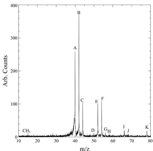
Figure 11: The mass spectra obtained from case 2. A: allene, B: propene/ketene, C: vinyl alcohol, D: mass 50, E: vinylacetylene, F: 1,3-butadiene (possible contribution from 1,2-butadiene), G: m/z 56. H= m/z 58, I: cyclopentadiene, J: m/z 68, K: benzene. Photon energy 10.0 eV.
