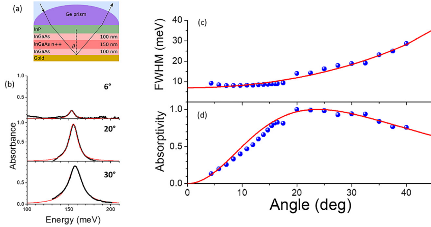
Figure 2: (a) Sketch of the sample and of the geometry used for reflectivity experiments. (b) Absorption spectra at three different internal angles (black lines) and Lorentzian fit of the resonances (red lines). (c) Full width at half the maximum (FWHM) of the absorption peak (blue symbols) as a function of the internal angle. Red line presents the calculated broadening, including radiative and nonradiative contribution. (d) Peak absorptivity extracted from the absorption spectra as a function of the angle, compared with the calculated one (red line) by using Eq. (3).
