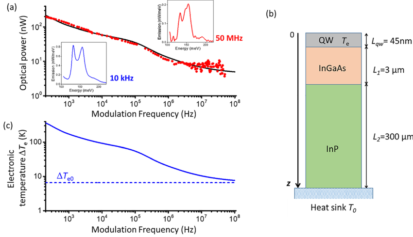
Figure 4: (a) Emitted power as a function of the modulation frequency (dots). The solid line is a result of modeling as described in the main text. The insets show two typical spectra for modulation frequency of 10 kHz and 50 MHz. (b) Schematic of semiconductor layers from the quantum well down to the heat sink used for our thermal model. (c) Estimations of the frequency-modulated part of the excess electronic temperature \Delta T_e(\omega) resulting from Eq. (9). The dashed line is the result of a simplified model where the effect of the semiconductor substrate has been neglected.
