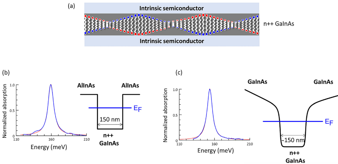
Figure 1: (a) Sketch of the system: a highly doped GaInAs layer embedded between two intrinsic semiconductor layers sustains a Berreman mode characterized by a dipole along the growth direction. (b) and (c) Conduction band profile and normalized absorption spectrum measured at 10^\circ internal angle (blue line) for a sample in which the two intrinsic layers are (panel b) AlInAs barriers or (c) intrinsic GaInAs layers. Red lines are Lorentzian fit of the absorption spectra.
