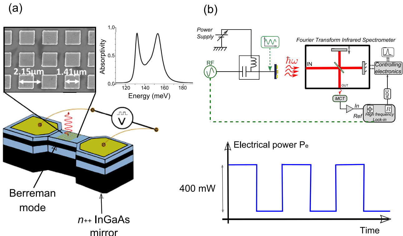
Figure 3: (a) Sketch of the device fabricated for thermal emission experiments. It consists of a 50 \times 50 \mu\text{m}^2 mesa with a top grating for the extraction of incandescent emission. In order to electrically excite the thermal emission, two lateral Ti/Au contacts ( 125 \times 100 \mu\text{m}^2 ) have been evaporated on the GaInAs layer sustaining the Berreman mode, after inductively coupled plasma reactive ion etching. The top part of the panel presents a scanning electron microscope image of the grating, with its characteristic dimensions, and the calculated absorption spectrum, displaying two polariton modes with almost unity peak absorptivity. (b) Sketch of the setup used for high frequency modulation of thermal emission. An electrical current is injected between the two lateral contacts. Its time modulation results in a modulation of the emitted power.
