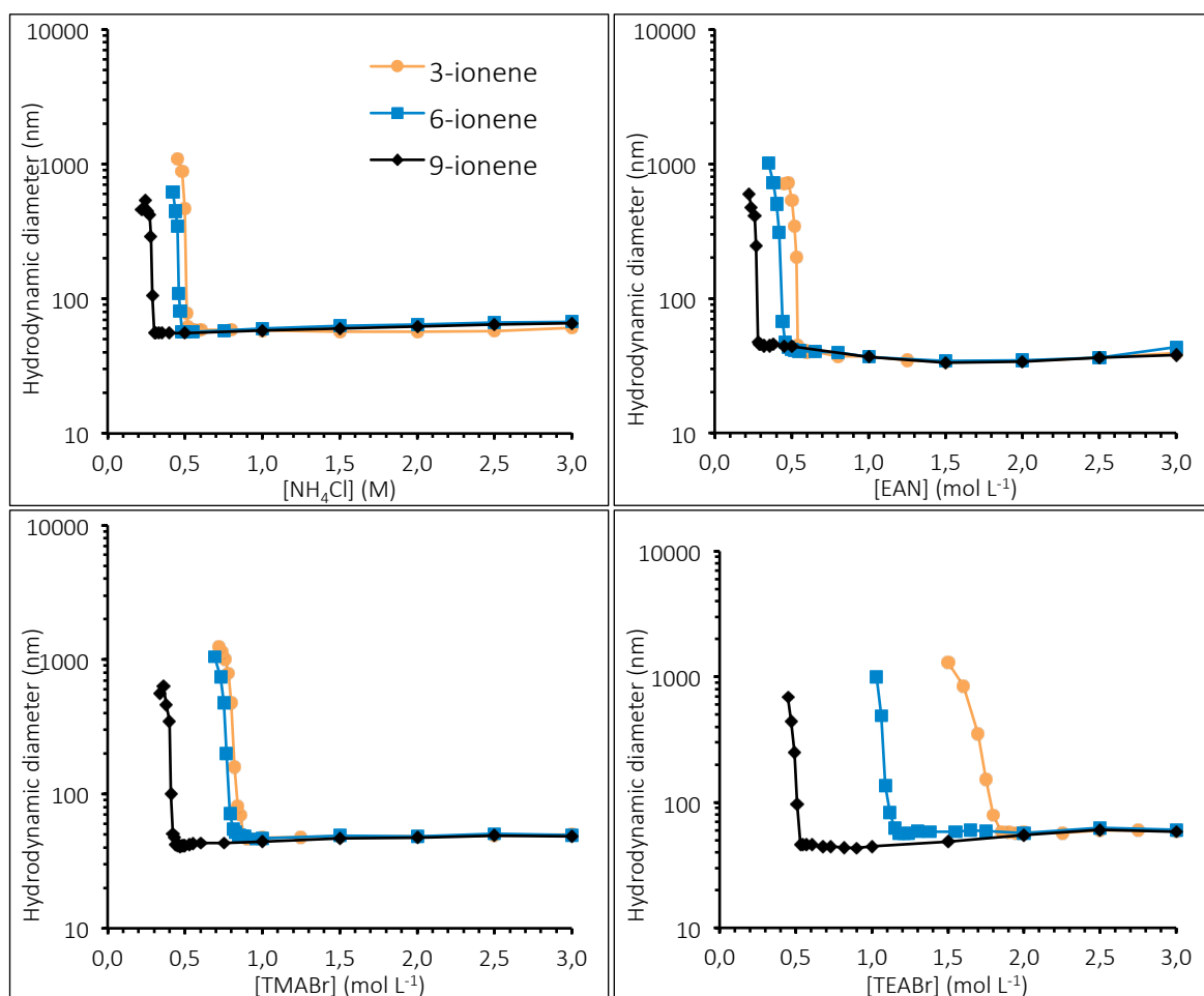
Figure 4. Dependence of the hydrodynamic diameter of CNPs in their mixtures with x-ionene (x=3, 6, or 9) PCs as a function of the salt concentration, for four different salts: NH 4 Cl, EAN, TMABr and TEABr. CNPs and PCs were prepared at initial concentrations of 0.5 wt % at charge ratios Z (Z = Z + /Z - ) 5.1, 4.1 and 3.4, respectively. The initial salt concentration was 3 mol L -1 in each case, the concentration was gradually decreased through a dilution process with distilled water, while pH was kept constant at 9.0.
