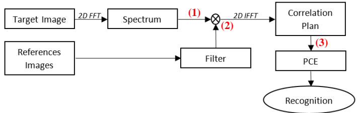
Fig. 5: Optical correlation principle
