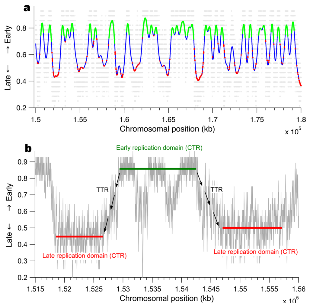
Figure 7. Replication timing profile generated by MM5. (a) The replication timing profile of a fictitious chromosome L = 200 Mbp ( N_0 = 1231 , J = 287 \text{ s}^{-1} , \theta = 0.46 , P_{in} = 0.34 , P_{local} = 0.34 , P_{out} = 0.01 , d = 138 kb). The grey dots are raw data and the blue line is the loess-smoothed curve. The green filled circles represent early firing origins and the red filled circles the late ones. (b) Replication timing profile for chromosomal positions [1.515, 1.56] \times 10^5 kb. The profile can be segmented into plateaus of early and late constant timing regions separated by timing transition regions.
