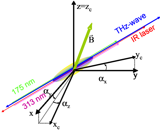
Fig. 1. The experimental setup and the reference coordinate frames.
