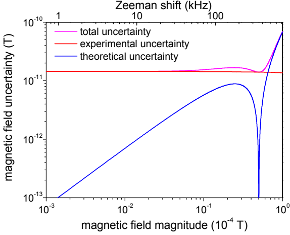
Fig. 2. Total uncertainty (magenta line), the contribution from the frequency measurement (red line), and the contribution from the theoretical calculation (blue line) of the magnitude of the magnetic field measured by Zeeman spectroscopy of the |v,L,F,S,J,J_z\rangle = |0,0,1,2,2,-2\rangle \rightarrow |0,2,1,2,4,0\rangle transition of \text{HD}^+ . The frequency uncertainty is estimated with the quantum projection noise-limited instability for a single-ion experiment with integration time 1 s and cycle time 1 s.
