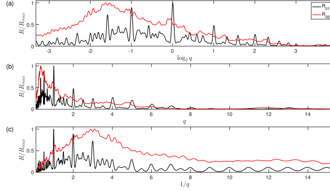
Fig. 8 Ratio distributions of voice signals ((1) #008 and (2) #169) and their frequency-matched Dirac comb models ( R_{0i} ). (a) Correlations of the frequency distribution \langle R_{0i} \rangle = R[\mathcal{S}_{0,j}, \langle \mathcal{S}_j^{(Q)} \rangle_t](\log q) ( j = 1, 2 , Q = 64 ) with their reference comb frequency distributions (defined in the text). These correlations have been normalised to their maximum for ease of comparison. (b, c) Plot of R[\mathcal{S}_{0,j}, \langle \mathcal{S}_j^{(Q)} \rangle_t] versus q for q > 1 (b) and 1/q for q < 1 (c).
