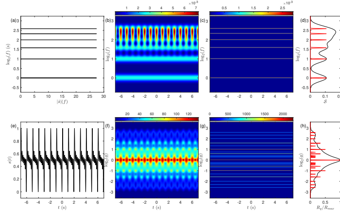
Fig. 5 Analysis of a model signal defined as the sum of 6 sine functions s(t) = \sum_1^6 \sin(2\pi f_i t) , with f_i = i f_1 constant. (a) Plot of \log(f(t)) . (b) \mathcal{S}^{(8)}(\log f, t) , computed for Q = 8 . (c) \mathcal{S}^{(128)}(\log f, t) , computed for Q = 128 . (d) \mathcal{S}^{(Q)}(\log f, t = 0) . (e) Temporal signal s(t) in the time window [-6.5\text{s}, 6.5\text{s}] . (f) R[\mathcal{S}^{(8)}, \mathcal{S}^{(8)}](\log q, t) . (g) R[\mathcal{S}^{(128)}, \mathcal{S}^{(128)}](\log q, t) . (h) R[\mathcal{S}^{(Q)}, \mathcal{S}^{(Q)}](\log q, t = 0) . In (d) and (h) the plots for Q = 8 (resp. 128) are coloured in black (resp. red). R[\mathcal{S}^{(Q)}, \mathcal{S}^{(Q)}](\log q, t) is defined in Eq. (26).
