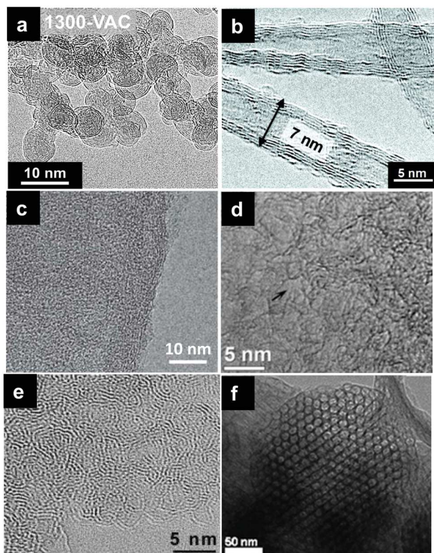
Fig. 3 Transmission electron micrographs (TEM) of various carbons with several dimensionalities for EDLCs: (a) OLCs, 94 (b) CNTs, 76 (c) graphene, 92 (d) ACs, 95 (e) CDCs, 65 and (f) TCs, 96
