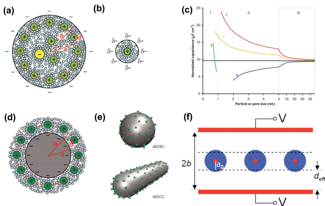
Fig. 6 Schematic illustrations (top views) of (a) an electric double-cylinder capacitor based on mesopores and (b) an electric wire-in-cylinder capacitor based on micropores.
