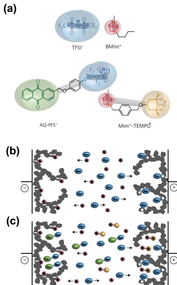
Fig. 16 (a) Structure of the biredox ionic liquid mentioned above. (b) and (c) Illustrations of the charge storage for pure IL and biredox IL, respectively.
