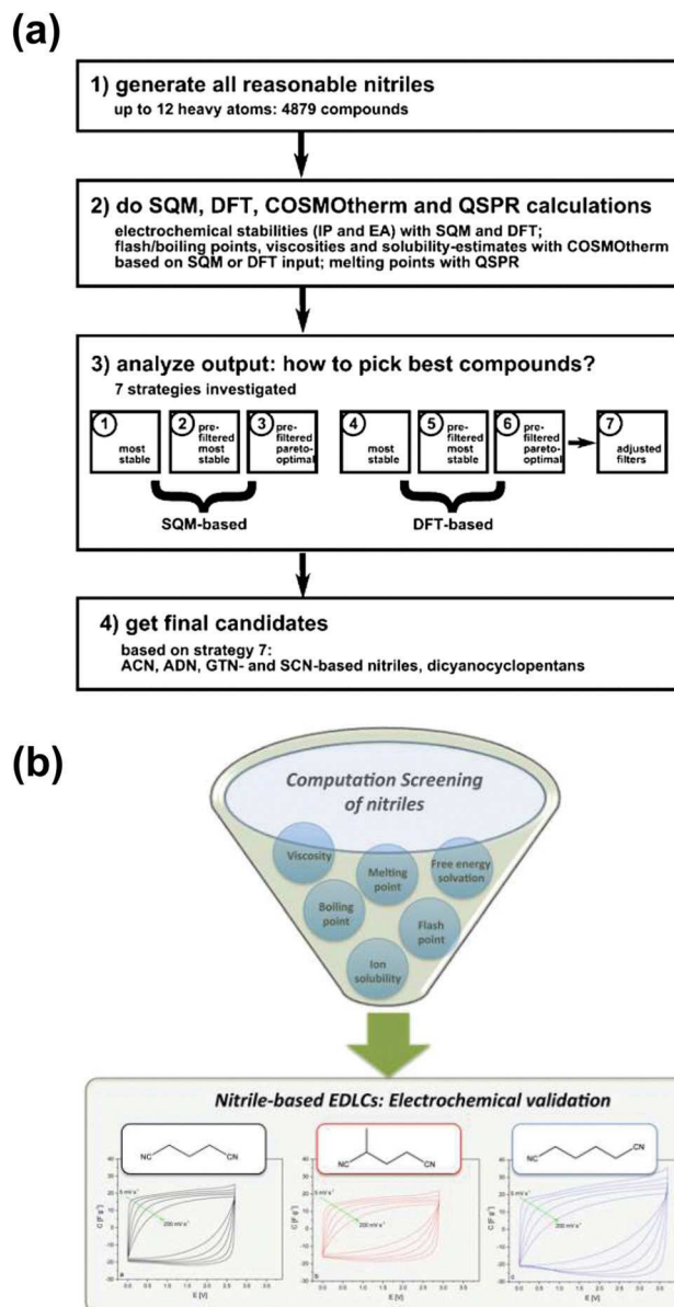
Fig. 15 (a) The screening strategy based on computational methods. (b) An illustration abstract for selecting a new solvent for supercapacitor applications.
