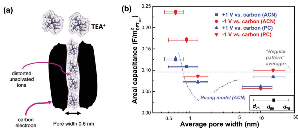
Fig. 5 (a) Illustration of the polarization-induced distortion of TEA + ions in pores with a size of 0.6 nm.
