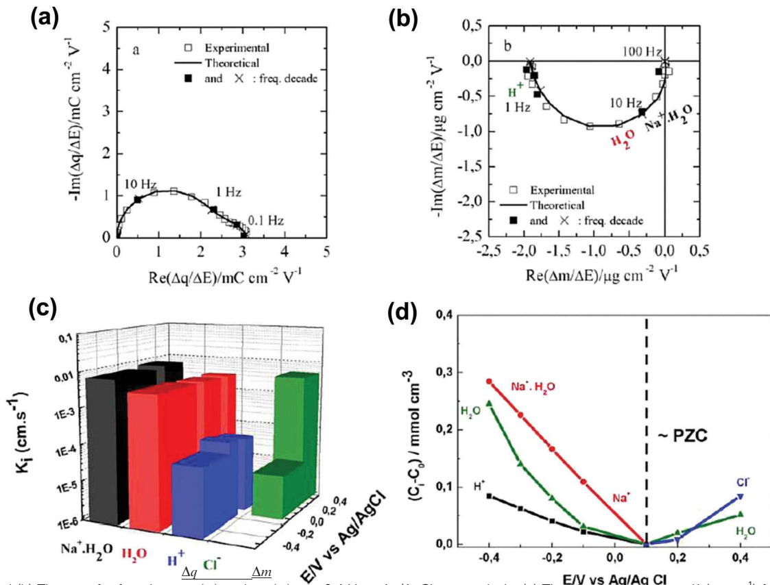
Fig. 8 (a) and (b) The transfer functions \omega and \omega at -0.4 V vs. Ag/AgCl, respectively. (c) The kinetic parameters K_i ( \text{cm}\cdot\text{s}^{-1} ) for each ion at SWCNT based thin films as a function of potential in 0.5 M NaCl at pH = 7.
