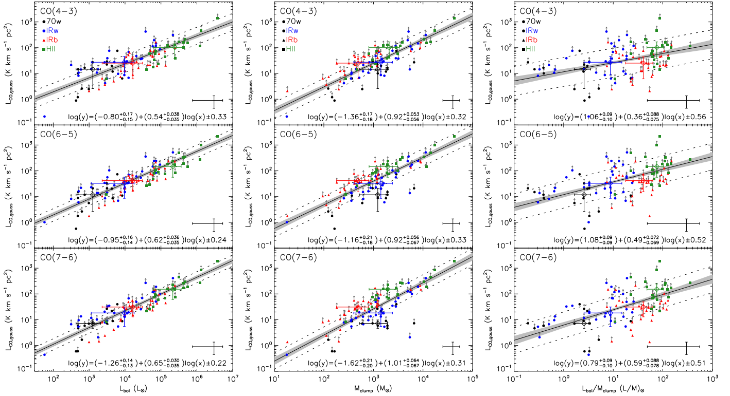
Fig. C.4. Line luminosity of the CO (4–3) ( upper panels ), CO (6–5) ( middle panels ) and CO (7–6) emission ( bottom panels ) versus the bolometric luminosity ( left panels ), the mass of the clumps ( middle panels ) and the L/M ratio ( right panels ) of the TOP100 sources. The median values for each class are shown as open diamonds and their error bars correspond to the absolute deviation of the data from their median value. Points having an upward arrow indicate a self-absorption feature in the spectrum convolved to 13''.4 and correspond to a lower limit. The typical error bars are shown at the bottom right side of the plots. The black solid line is the best fit, the light grey shaded area indicates the 68% uncertainty, and the dashed lines show the intrinsic scatter ( \epsilon ) of the relation.
