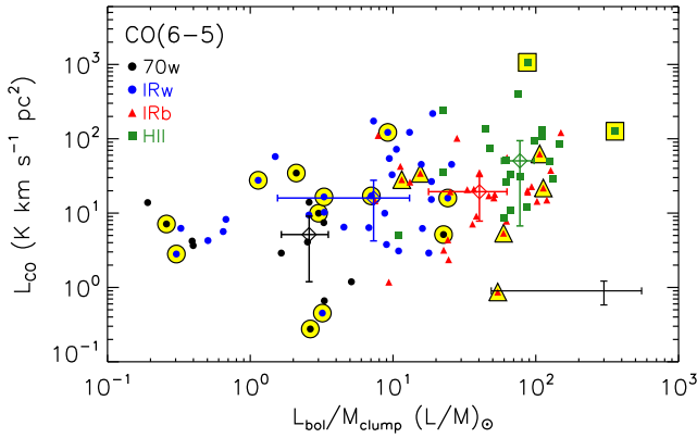
Fig. 9. Same as the right panel of Fig. 7, but displaying L_{CO} of the CO(6–5) line as a function of the L/M ratio of the TOP100 sources. Data points highlighted in yellow indicate those sources from which no signs of self-absorption features were identified in the spectrum convolved to 13''.4 .
