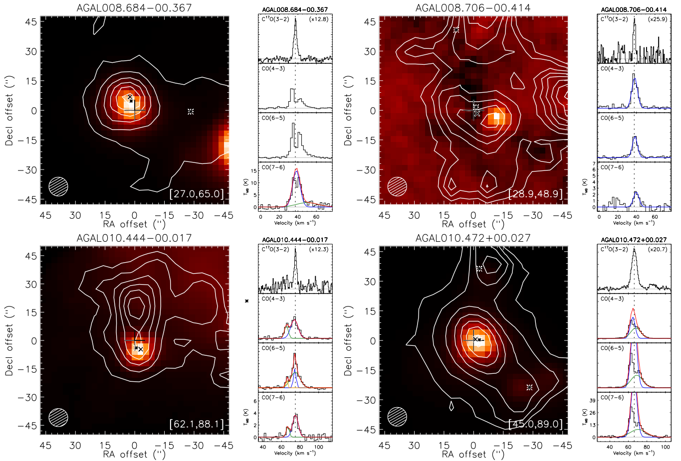
Fig. B.1. Left panels: false-colour Herschel /PACS images at 70 \mu\text{m} overlaid by the CO(6–5) emission contours towards the TOP100 source. The CO contours correspond to the emission integrated over the full-width at zero power (FWZP) of the CO(6–5) profile, the velocity range shown in the bottom right side of the image, and the contour levels are shown from 20% to 90% of the peak emission of each map, in steps of 10%. The (0,0) position of the map is shown as a + symbol, the position of the CSC source from Contreras et al. (2013) is shown as a \times symbol and the dust continuum emission peaks from Csengeri et al. (2014) are shown as asterisks. Right, from top to bottom panel: C 17 O(2–1) or C 18 O(1–0) from Giannetti et al. (2014), CO(4–3), CO(6–5) and CO(7–6) profiles towards the TOP100 sample, convolved into a fixed beam size of 13''4 (shown in black) and their fitted Gaussian components. The narrower Gaussian component fitted to the data is shown in blue, the second and broader component is shown in red and the third component is shown in yellow. The sum of all Gaussian components is shown in red, except for the cases where a single component was fitted. The vertical dashed black line is placed at the rest velocity ( V_{1sr} ) of each source. The horizontal filled grey line displays the baseline of the data.
