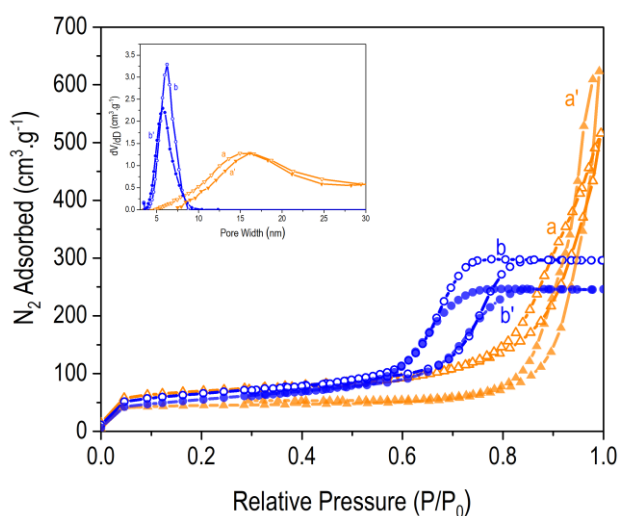
Figure 1. \text{N}_2 physisorption isotherms and pores sizes distribution (in inset) after degassing at 250 \text{ }^\circ\text{C} of the (a,b) calcined and (a',b') reduced materials: (a,a') \text{Ni}_{5\text{wt}\%}\text{-Al}_2\text{O}_3\text{-MOF} and (b,b') \text{Ni}_{5\text{wt}\%}\text{-Al}_2\text{O}_3\text{-EISA} .
