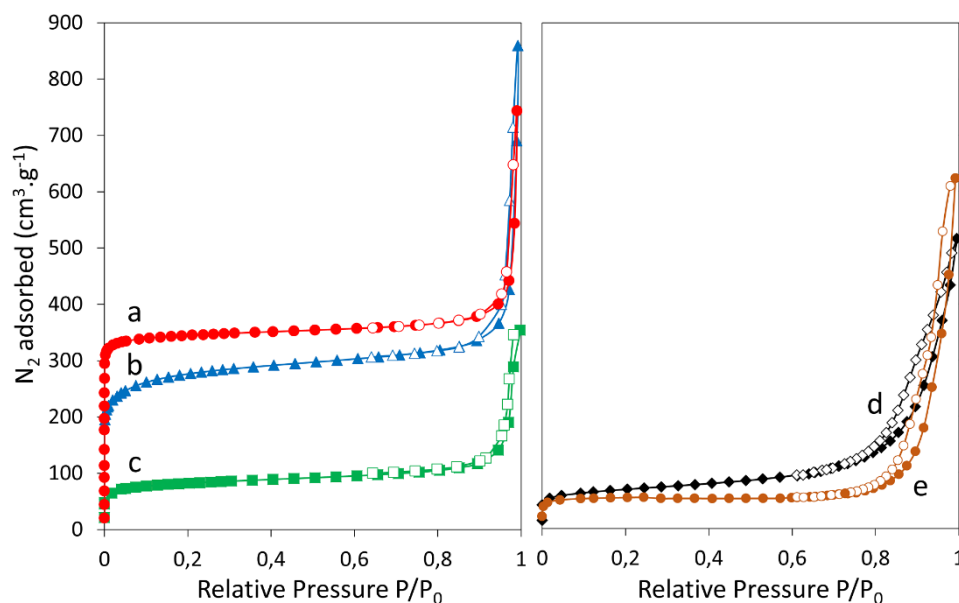
Figure 3. N_2 physisorption isotherms after degassing at 120^\circ \text{C} of: (a) freshly activated MIL (red spheres), (b) rehydrated MIL (blue triangles), (c) Ni/MIL (green squares), (d) NiAl_{MIL} (black diamonds) and (e) Ni^0Al_{MIL} (brown spheres). Filled and empty symbols correspond to adsorption and desorption isotherms, respectively.
