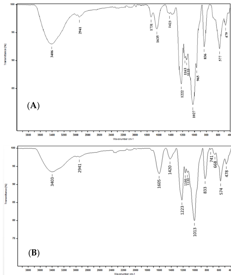
Figure 2. ATR-FTIR spectra of sulfated polysaccharides from (A) B. bifurcata (BBF) and (B) F. spiralis (FSF).
