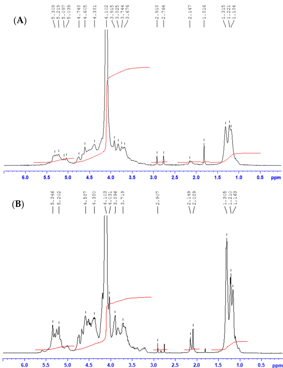
Figure 1. ^1\text{H} NMR spectra of sulfated polysaccharides from (A) B. bifurcata (BBF) and (B) F. spiralis (FSF) at 60 °C in \text{D}_2\text{O} solution.
