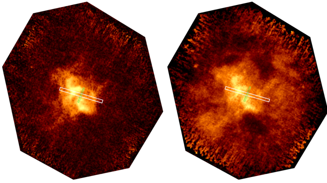
(a) RS Pup
