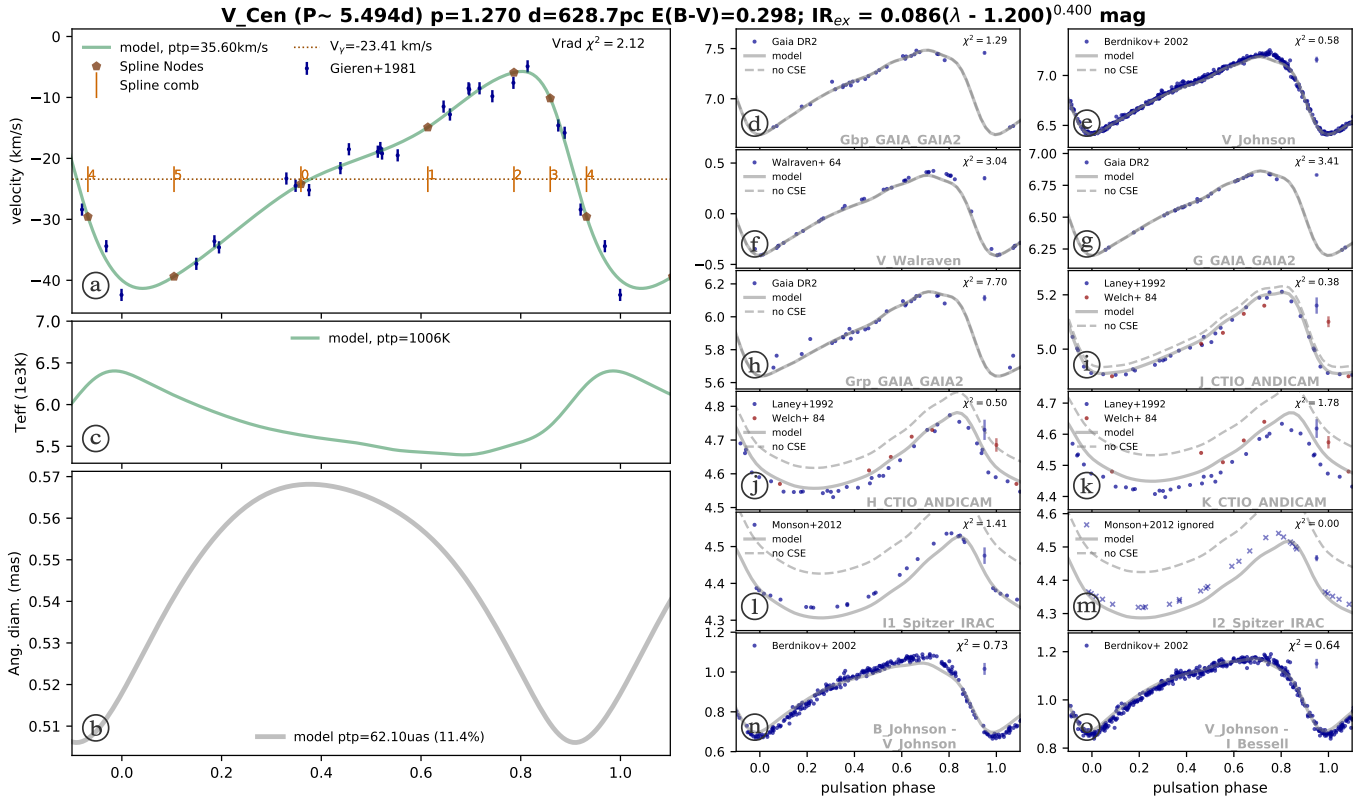
Fig. A.2. The SPIPS results of V Cen. Velocity: Gieren (1981) . Effective temperature: No data. Angular diameter: No data. Photometry: Walraven et al. (1964) , Welch et al. (1984) , Laney & Stobie (1992) , Berdnikov & Turner (2002b) , Monson et al. (2012) , Gaia Collaboration (2018) .
