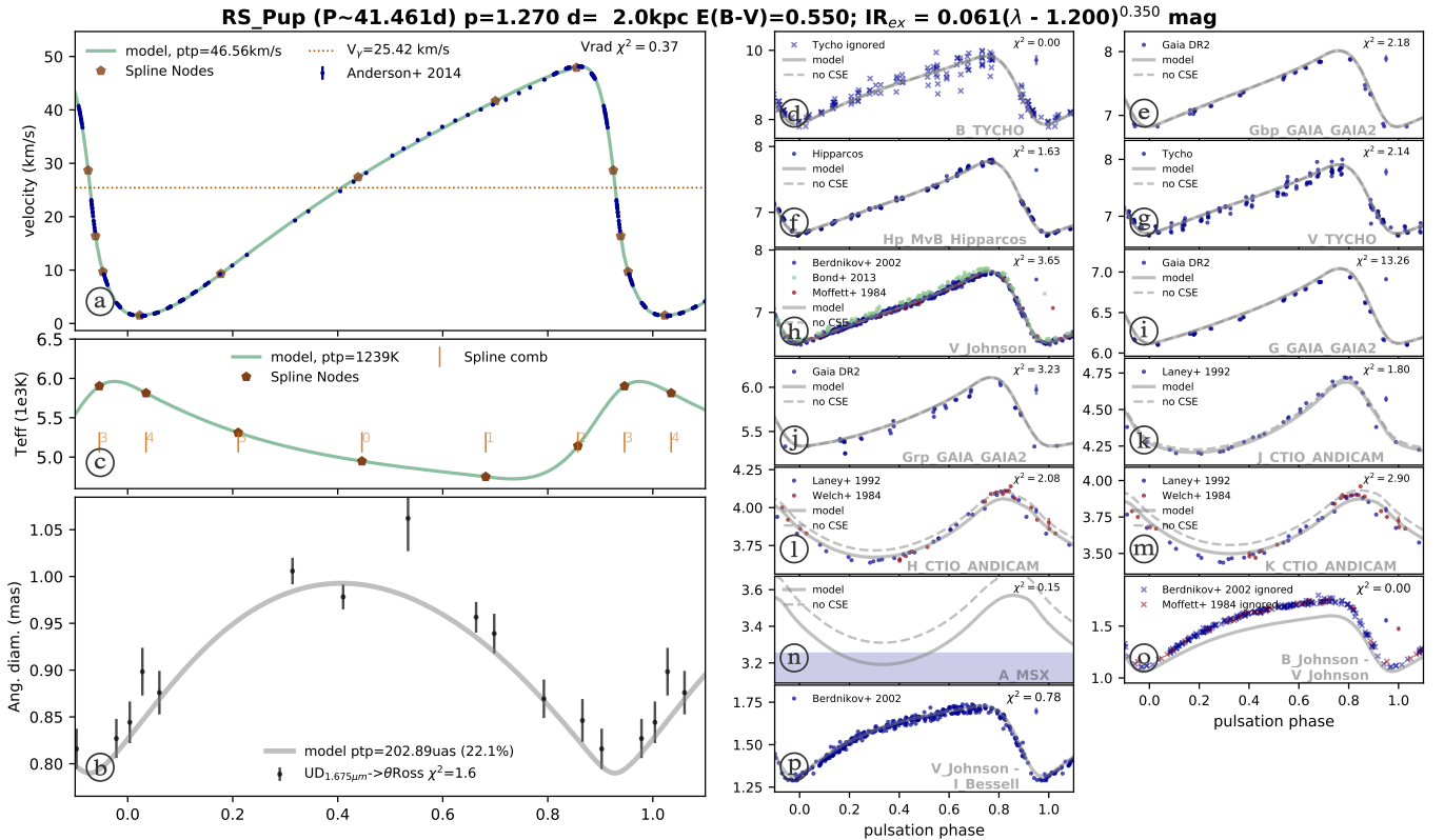
Fig. A.3. The SPIPS results of RS Pup. Velocity: Anderson (2014) . Effective temperature: No data. Points are nodes for a spline interpolation. Angular diameter: Kervella et al. (2017) . Photometry: Moffett & Barnes (1984) , Welch et al. (1984) , Laney & Stobie (1992) , ESA (1997) , Price et al. (2001) , Berdnikov & Turner (2002a) , Gaia Collaboration (2018) .
