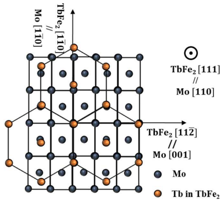
Figure 9. Superimposition of the (111) TbFe 2 (gold) and (110) Mo (blue) surface lattices in R30-orientation.
