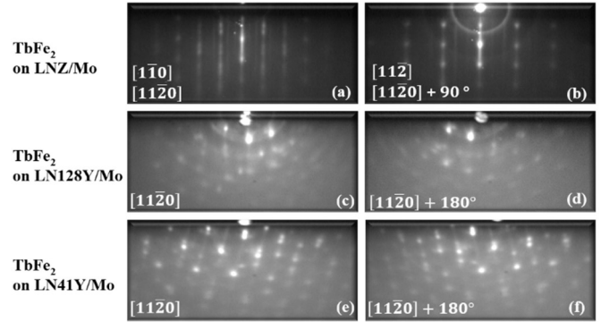
Figure 7. RHEED images collected after the deposition of 50 nm thick TbFe 2 films on LN Z /Mo (a and b), on LN128Y/Mo (c and d) and on LN41Y/Mo (e and f). Azimuthal positions refer to the LN substrate and to the TbFe 2 lattice in the case of LN Z substrate.
