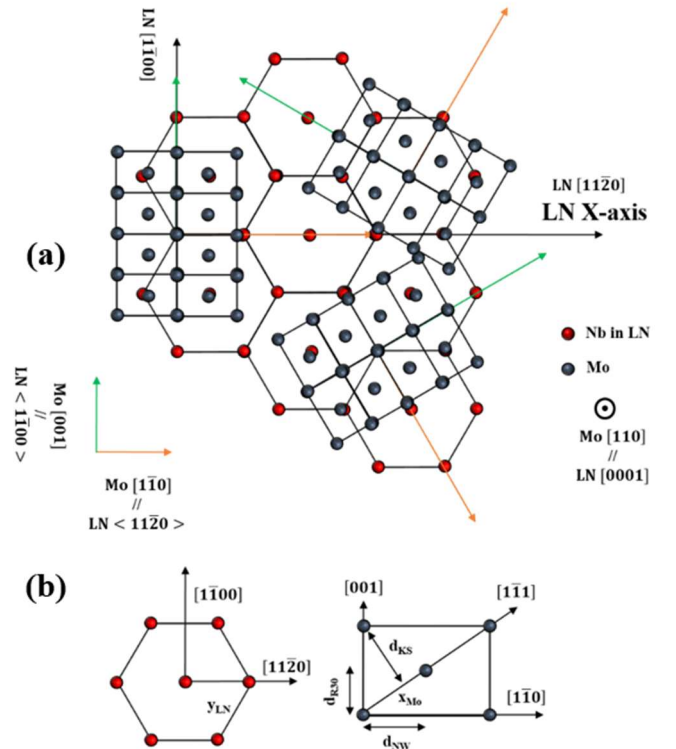
Figure 6. (a) Superimposition of three (110) Mo domains (blue) on (0001) LN (Nb atoms of LN in red). (b) sketch for (0001) hcp and (110) bcc planes with nearest-neighbor distances y_{\text{LN}} and x_{\text{Mo}} . d_{\text{KS}} , d_{\text{NW}} and d_{\text{R30}} are the distances between densely-packed rows of the bcc (110) plane corresponding to the KS, NW and R30 orientations.
