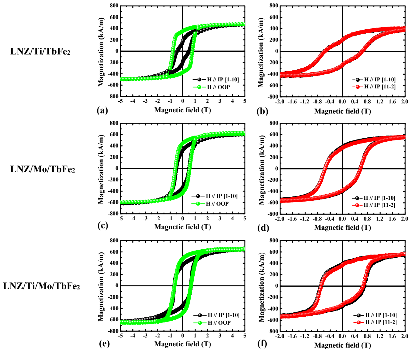
Figure 6. Hysteresis loops measured at room temperature with the magnetic field applied IP along two orthogonal directions (black and red) and OOP (green) for 50 nm thick \text{TbFe}_2 layers deposited on different templates (single buffer layers (Ti (a and b) and Mo (c and d)) and double buffer layers (Ti/Mo (e and f)).
