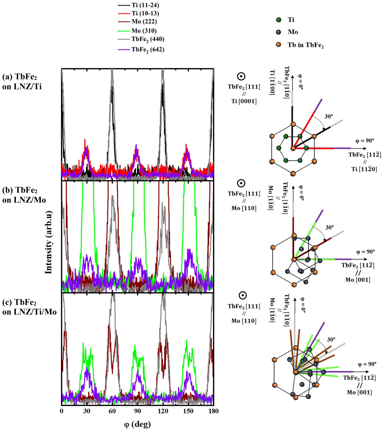
Figure 4. \phi scans for asymmetrical reflections measured for (a) LNZ/Ti/TbFe 2 , (b) LNZ/Mo/TbFe 2 and (c) LNZ/Ti/Mo/TbFe 2 The sketches on the right are superimpositions of the corresponding planes deduced from the \phi scans. For the sake of clarity, only three of the six Mo domains are presented on the bottom sketch
