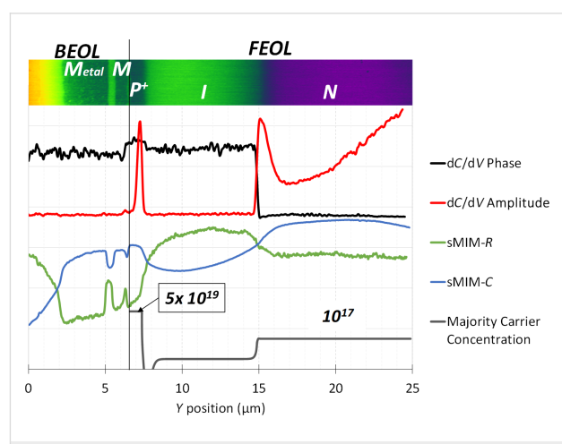
Figure 5: Depth profiles ( \partial C/\partial V phase, \partial C/\partial V amplitude, sMIM-R, and sMIM-C) along the PIN structure compared with simulated concentration values for the majority carriers.
