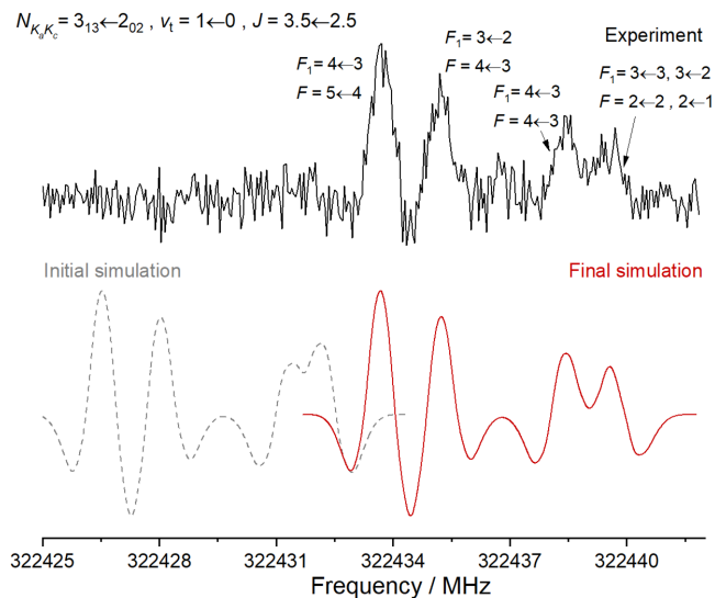
Fig. 3. Overview of one cluster of lines in the \nu R_0(2) rotational transition of \text{CH}_2\text{OH} . The black trace corresponds to the experimental survey and it is compared with 300 K spectral simulations performed using the initial (refit, in gray) and final (in red) set of parameters. The presented experimental spectrum results from the subtraction of two recordings, without and with a permanent magnet, so that only transitions arising from open-shell species are visible. The full width at half maximum of both spectral simulations were chosen to reproduce the experimental signal at best.
