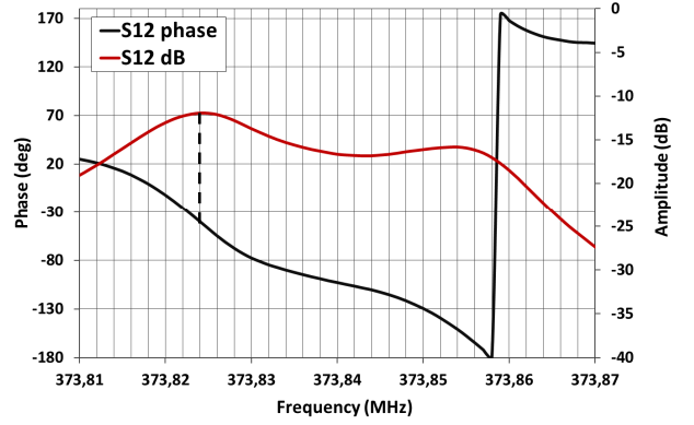
Fig. 5. S_{12} parameters of the tested HBAR around 373 MHz.
