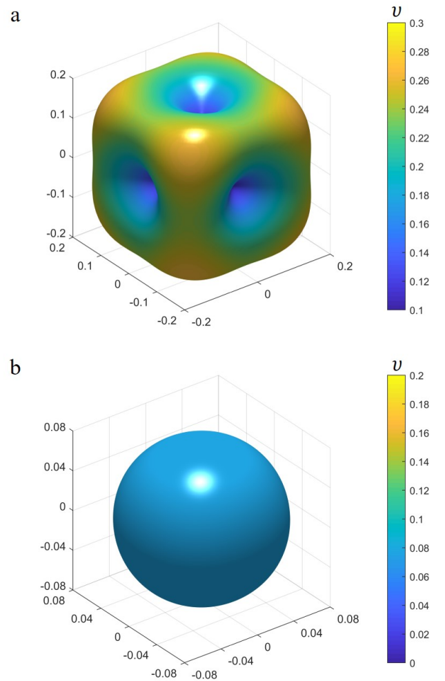
Figure 4: Three dimensional polar plot of the Poisson’s ratio following by Eq. (9) for (a) the initial structure and (b) the optimal isotropic structure 1.
