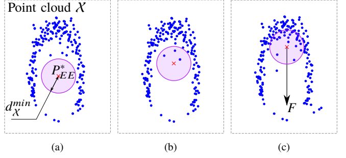
Fig. 4. Computation of the repulsive force used as a switch between the "Translating" and "Rotating" tasks. In (a), the detected contour of the environment along with the circle of radius d_\chi^{\min} are represented. In (b), some points of the contour move inside the circle, creating a repulsive force visible in (c).
