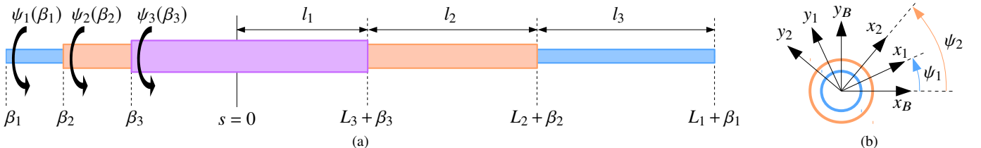
Fig. 1. (a) 3-tube CTR straightened for ease of understanding, and (b) cross-sectional view of link 2 of the CTR with the orientation of the material base frames of tubes 1 and 2 relative to the Bishop frame.
