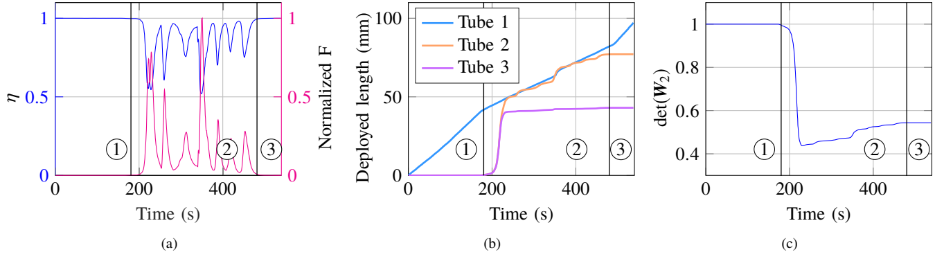
Fig. 6. (a) Normalized repulsive force F (filtered) and \eta , (b) inserted tube lengths, and (c) stability of the CTR over time, with the deployment steps identified and labeled, in the case of the simulation with deployment in the nasal cavity.
