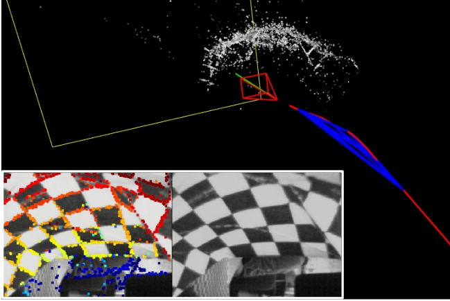
Fig. 10. Navigation in the origami tunnel. Top : reconstructed shape, with the red lines showing the camera trajectory. Bottom : images coming from the virtual camera, with and without the detected features.
