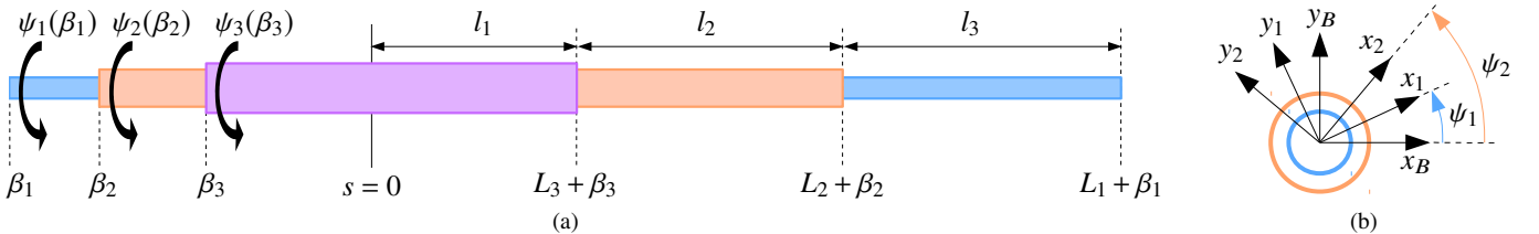
Fig. 1. (a) 3-tube CTR straightened for ease of understanding, and (b) cross-sectional view of link 2 of the CTR with the orientation of the material base frames of tubes 1 and 2 relatively to the Bishop frame.
