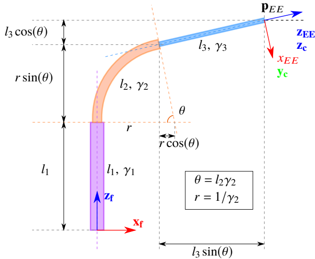
Fig. 2. Geometry of the CTR under consideration. l_i and \gamma_i are the length and curvature of i -th link of the CTR.
