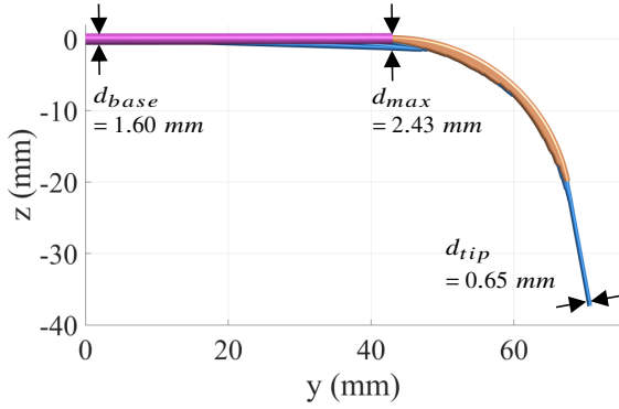
Fig. 8. Superposition of all intermediate CTR shapes adopted during deployment for the simulation, with measurements of the outer envelope. An approximate FTL deployment is observed.
