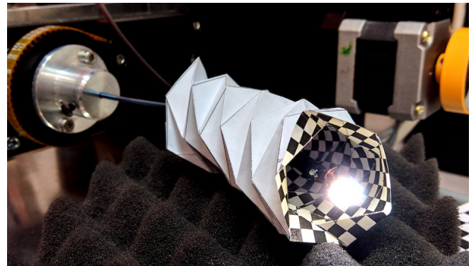
Fig. 12. CTR with the RGB camera attached at its distal end successfully navigating through the origami tunnel.
