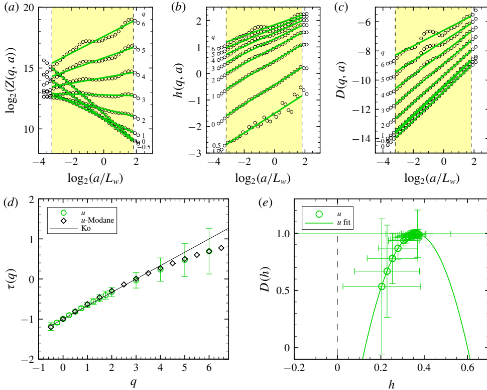
FIGURE 8. Same as figure 6 but for a stable atmospheric regime (run 27 in table 1).
