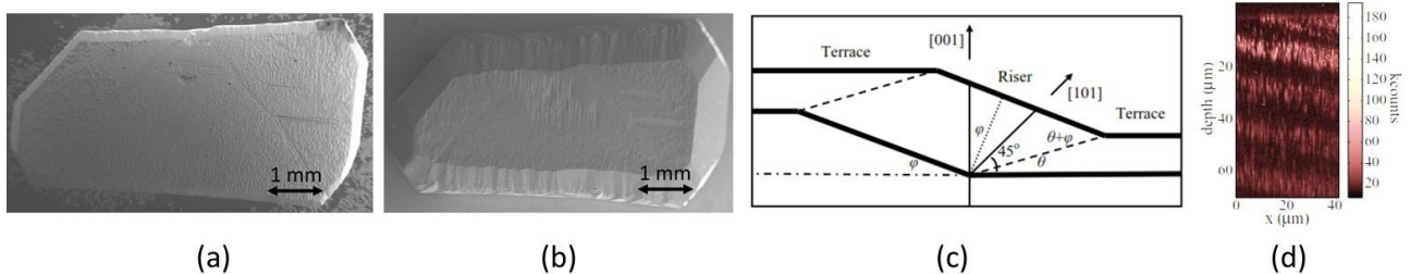
Figure 14. Surface morphology of a (110)-oriented CVD layer after a growth of (a) 6 hours ( 60\ \mu\text{m} ) and (b) 30 hours ( 300\ \mu\text{m} ). The top surface area has eventually decreased by a factor of 2. (c) Scheme of macro-steps formed at the surface of a [100]-oriented diamond film during growth where risers and terraces are identified. This image is adapted from Martineau et al. [240]. (d) Preferential incorporation of NVs at the risers of the steps with (110) orientation. This image is adapted from Pham et al. [241].
