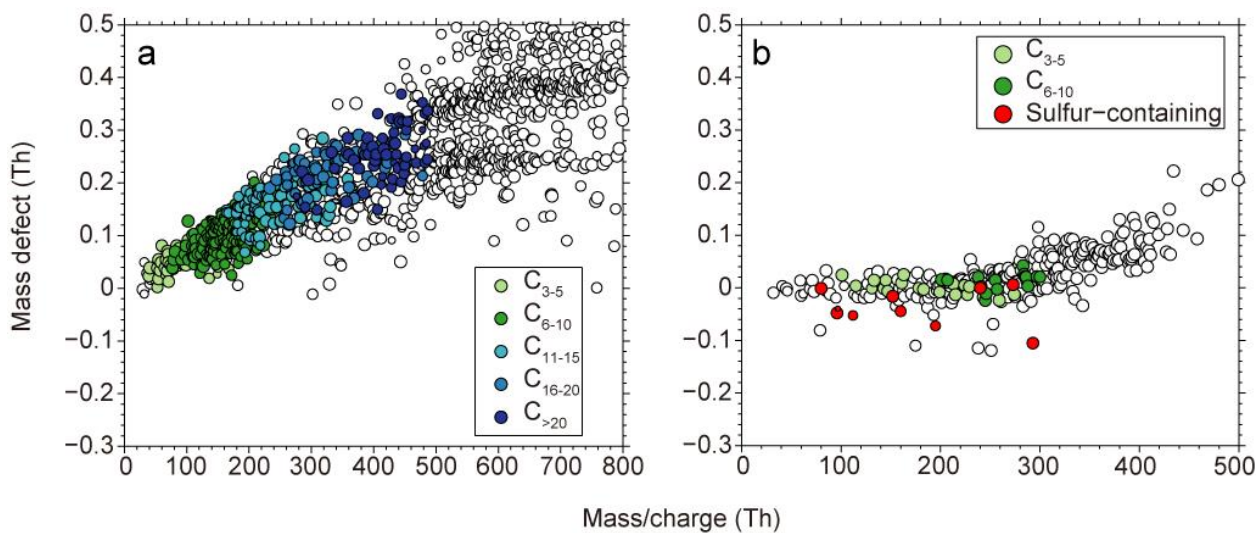
Figure 3. Chemical composition of the positive and negative ions (molecules and clusters)
