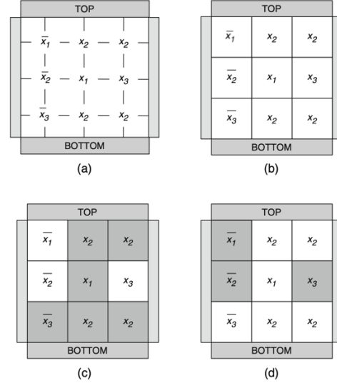
Fig. 1 A four terminal switching network implementing the function f = x_1x_2x_3 + x_1x_2 + x_2x_3 ; its corresponding lattice form b ; the lattice evaluated on the assignments 1,1,0 ( c ) and 0, 0, 1 ( d ), with grey and white squares representing ON and OFF switches, respectively
