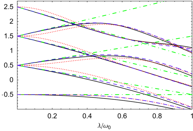
FIG. 1. Generalized rotating wave approximation applied to the Rabi Hamiltonian H_{\text{QRM}} . Comparison of RWA (dotted-dashed line), limit \Omega = 0 (dotted line), and GRWA (dashed line) with the exact spectrum (solid line). Reproduced with permission [60]. Copyright 2007, American Physical Society.
