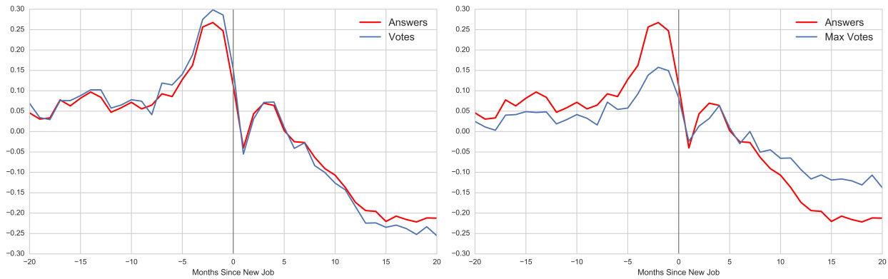
(A) Number of Answers vs. Votes received from Answers
