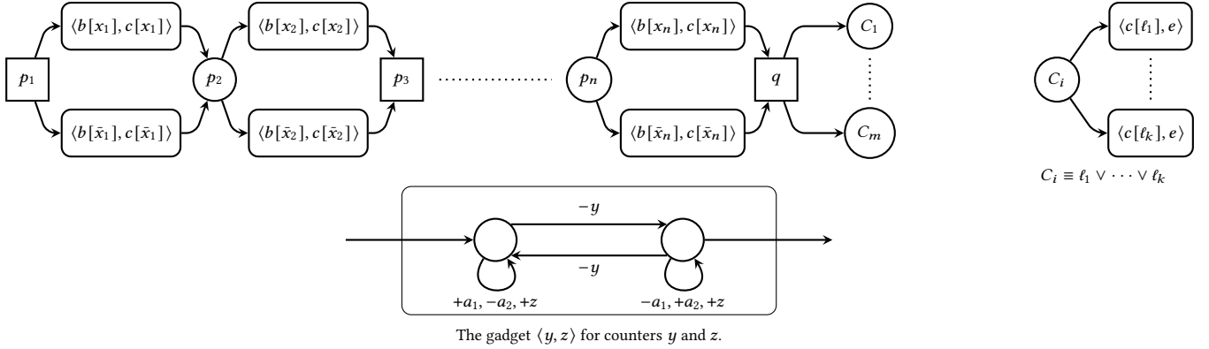
Figure 6. The problem whether \mathcal{L}_{\mathcal{A}} \in \mathcal{O}(n^2) for a given VASS game \mathcal{A} is PSPACE -hard.
