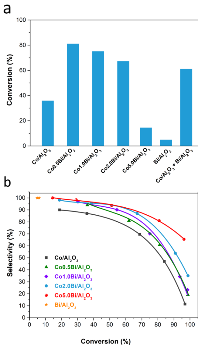
Figure 3 Catalytic conversion modification by Bi promotion (a) and selectivity-conversion curves (b) for liquid phase amination of 1-octanol over activated Co/Al 2 O 3 and bimetallic Co x Bi/Al 2 O 3 catalysts (1-octanol, 0.84 g; molar ratio of 1-octanol/NH 3 /H 2 = 1/4.5/0.85; P H 2 = 3 bar; catalyst amount, 100 mg; reaction temperature, 180 °C; time, 0-48 h; no solvent used).
