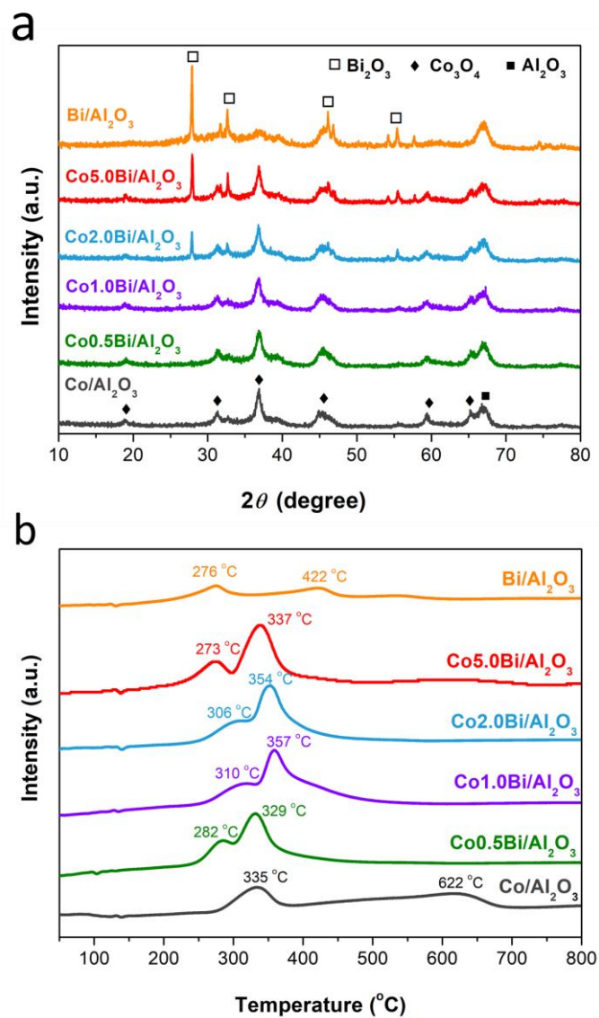
Figure 5 XRD patterns (a) and H 2 -TPR profiles (b) of oxidized Co/Al 2 O 3 , Bi/Al 2 O 3 and bimetallic Co x Bi/Al 2 O 3 catalysts.
