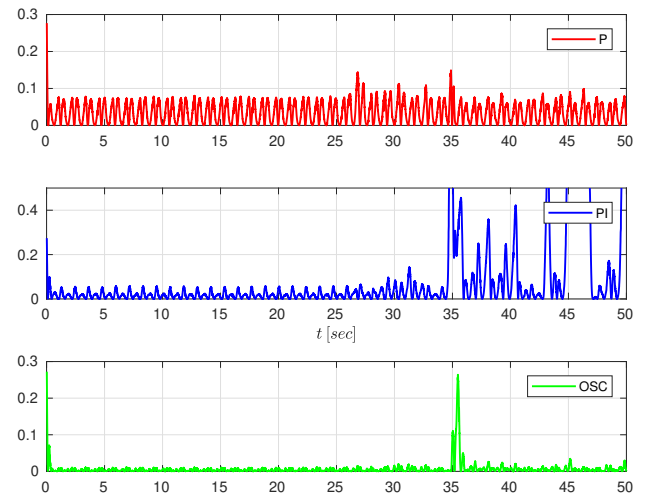
Fig. 12. Time behaviour of the Frobenius norm \|I - \tilde{H}\|_F of the proportional observer (red line), proportional-integral observer (blue line) and internal model based observer (green line).
