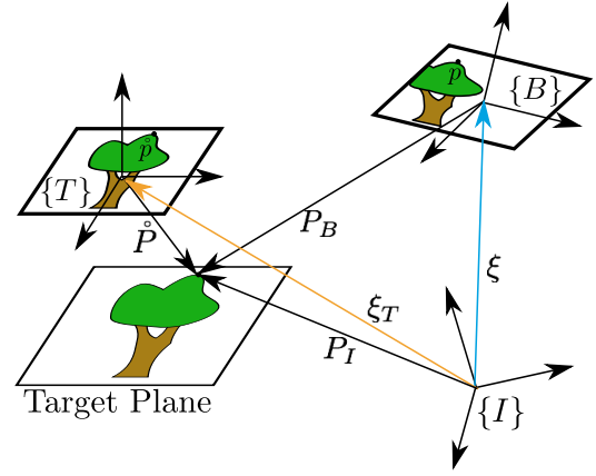
Fig. 1. Representation of a point of the planar surface in the inertial frame \{I\} , body-fixed frame \{B\} and target frame \{T\} .
