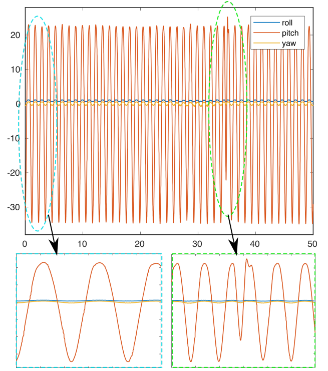
Fig. 11. Roll, pitch and yaw Euler angles of the oscillating platform.
