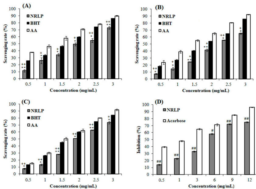
Figure 4. Antioxidant capacity of NRLP evaluated using (A) phospho-molybdenum, (B) hydroxyl and (C) DPPH radicals scavenging assays in different solutions and (D) the \alpha -amylase inhibition effect. Data are shown as means of three separate experiments. * p < 0.1 and ** p < 0.01 compared with the positive control ascorbic acid (AA). + p < 0.1 and ++ p < 0.01 compared with the positive control butylhydroxytoluene (BHT). # p < 0.05 and ## p < 0.01 compared with the positive control acarbose.
