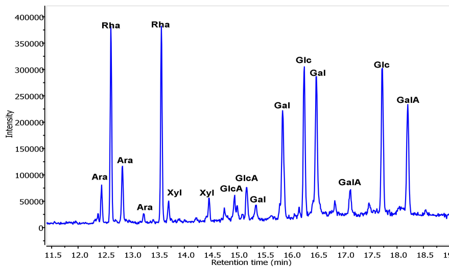
Figure 2. Gas Chromatography/Mass Spectrometry - Electronic Impact (GC/MS-EI) (70 eV) total ion chromatogram of trimethylsilyl- O -glycoside residues prepared from NRLP.
