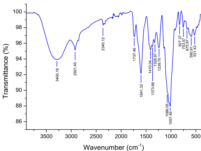
Figure 3. FTIR spectrum of NRLP.
